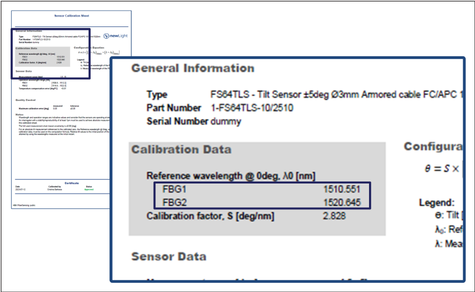
Fig. 2.11 Calibration sheet example - FBG wavelengths
