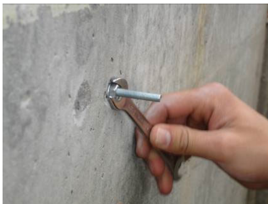
Fig. 2.3 Anchor tightening
