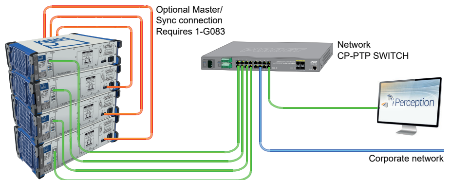
Figure 5: Multi mainframe
