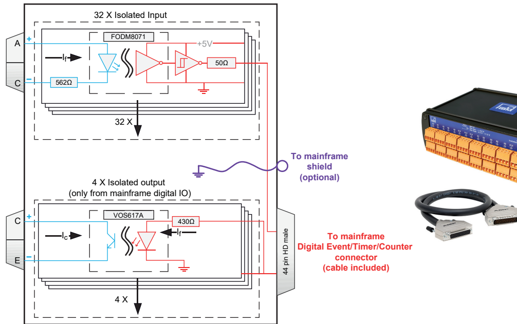
Figure 29: Block diagram and image
