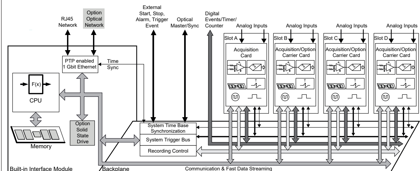
Figure 7: Block diagram
