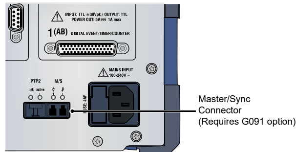
Figure 12: Master/Sync connector
