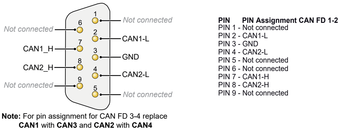
Figure 33: Pin assignment CAN FD Option
