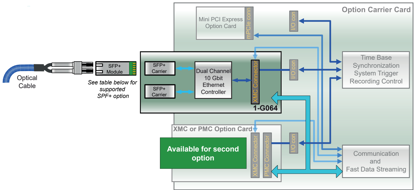
Figure 20: Block diagram 10Gbit Ethernet card, optical (G081 required)
