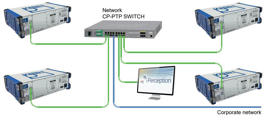
Figure 6: Multi mainframe (distributed)
