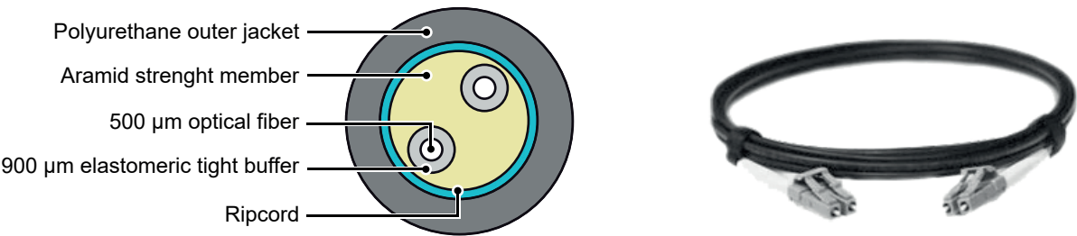
Figure 27: Block diagram and image
