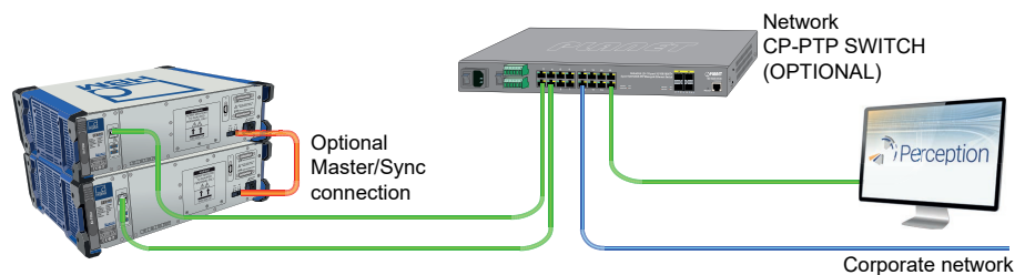
Figure 4: Dual mainframe
