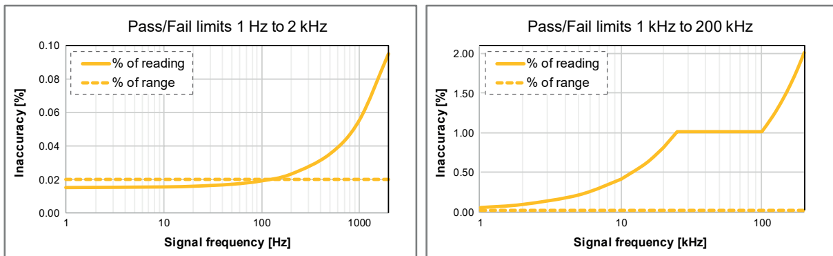
Figure 4: Power pass/fail limits (0.33 \Omega shunt), Wideband and 0.5 \leq Power Factor \leq 1
