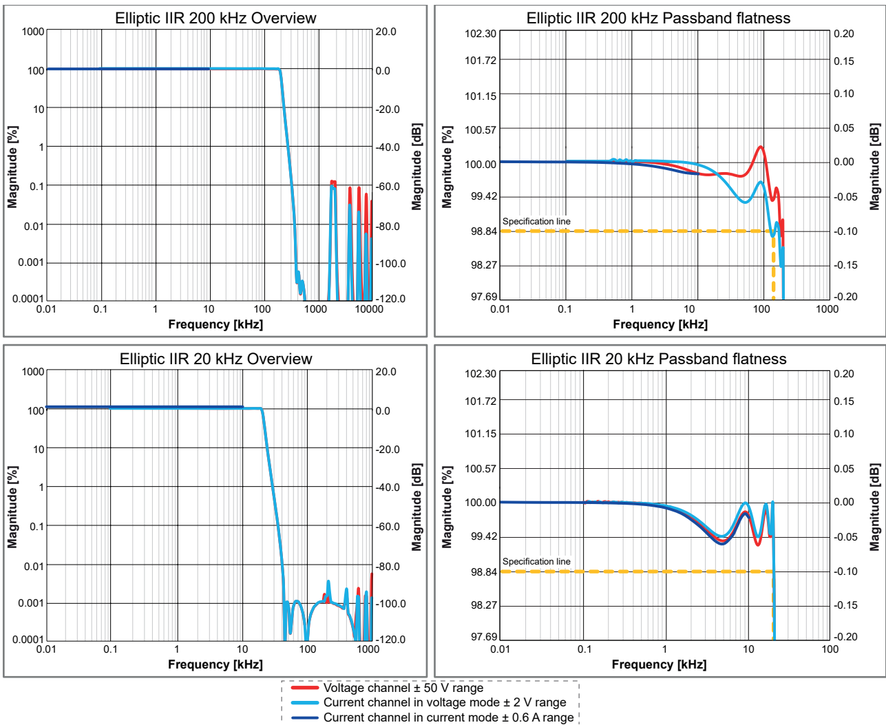
Figure 31: Representative Elliptic IIR examples (200 kHz for GN310B only; 20 kHz for GN310B and GN311B)
