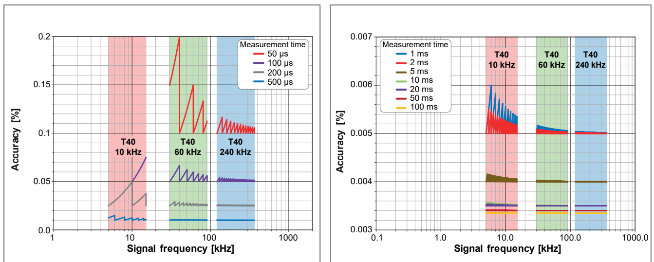
Figure 38: Torque operating range versus inaccuracy and measurement time
