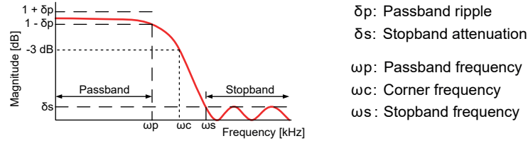
Figure 26: Digital Bessel IIR Filter (200 kHz for GN310B only; 20 kHz for GN310B and GN311B)
