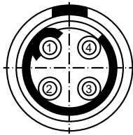
Figure 16: Cable connector soldering view
