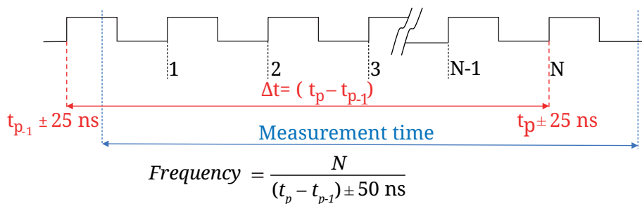
Figure 36: Frequency measurement
