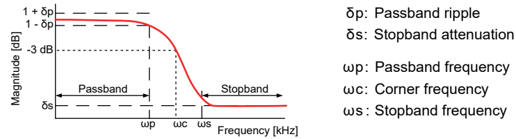
Figure 22: Bessel Filter
