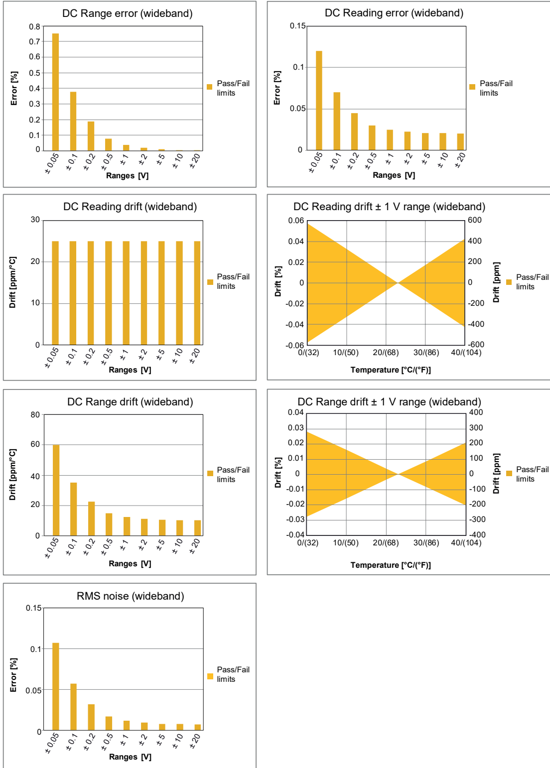
Figure 12: Wideband voltage mode specification
