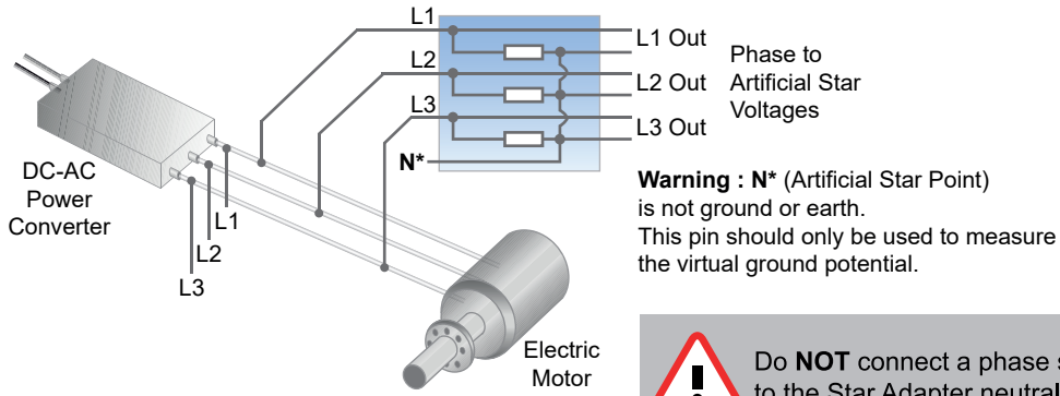
Figure 42: Three phase representative use of artificial star adapter
