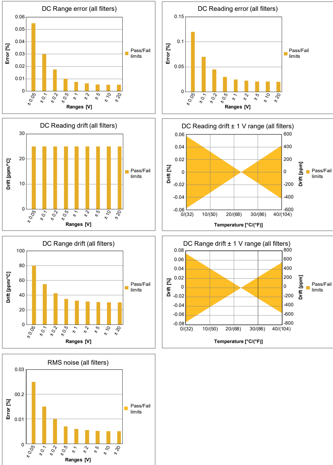
Figure 13: All filters used voltage mode specification
