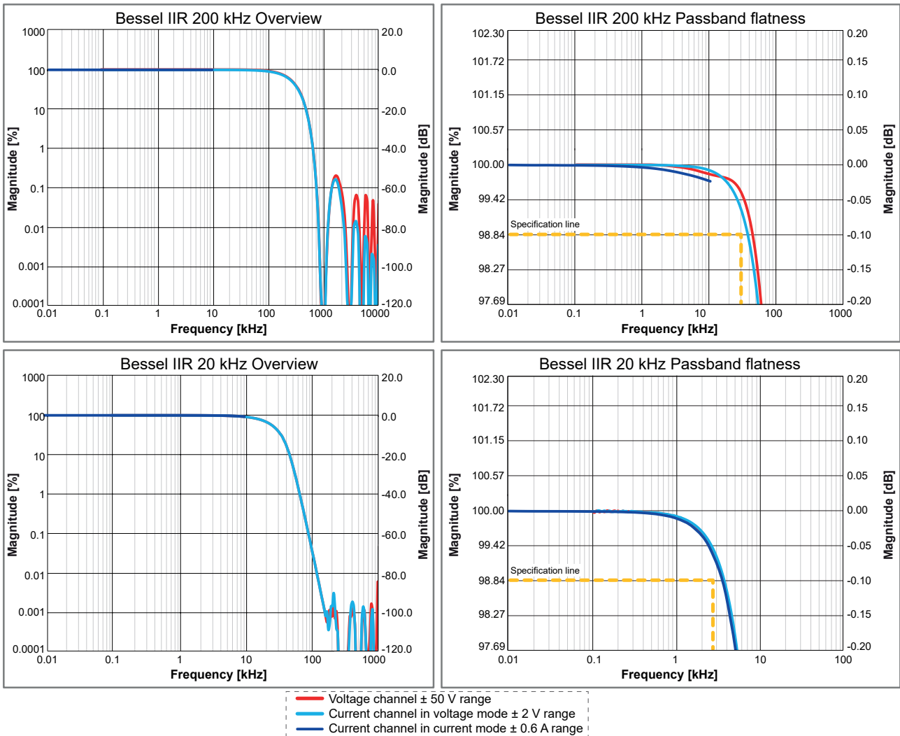
Figure 27: Representative Bessel IIR examples (200 kHz for GN310B only; 20 kHz for GN310B and GN311B)
