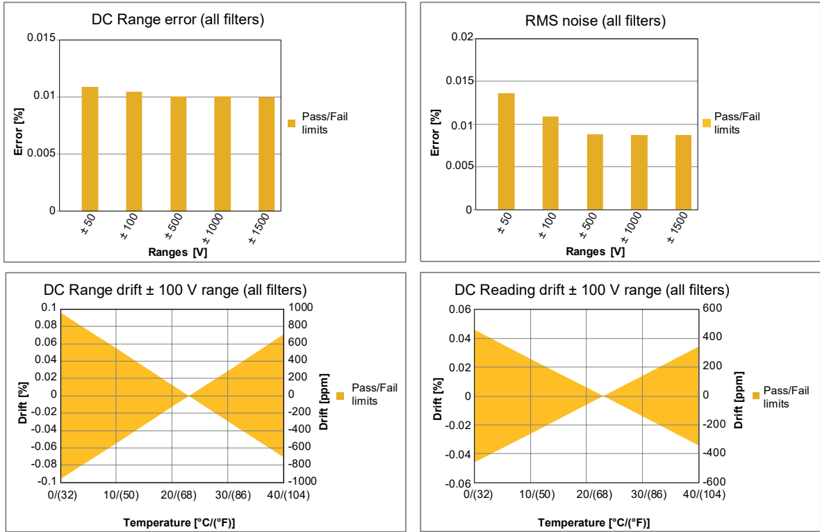
Figure 7: All filters used voltage specification
