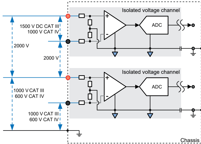
Figure 17: Voltage channels isolation ratings
