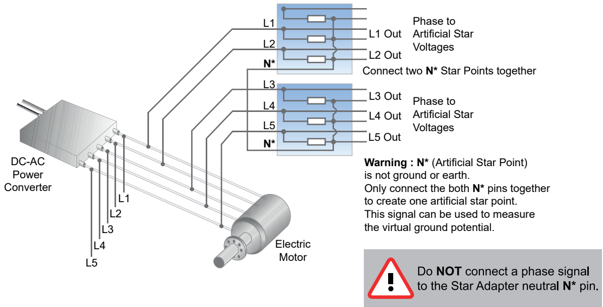
Figure 43: Five or more phase representative use of dual star adapter
