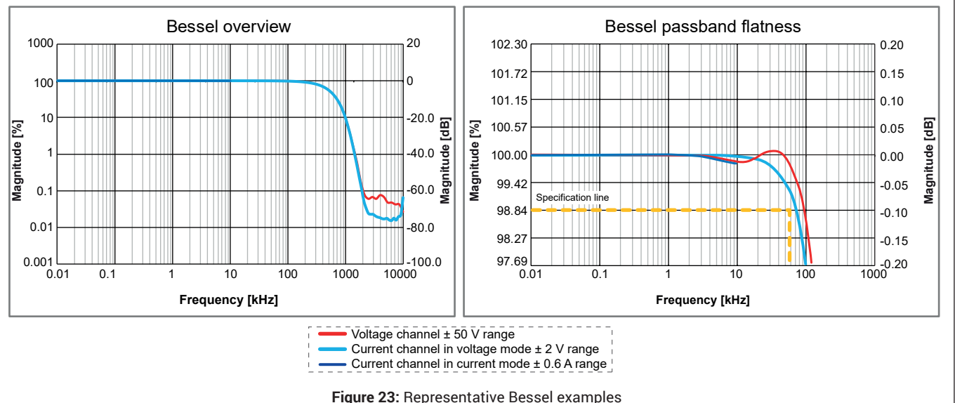
Figure 23: Representative Bessel examples
