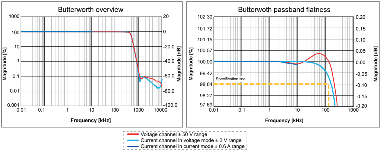
Figure 25: Representative Butterworth examples
