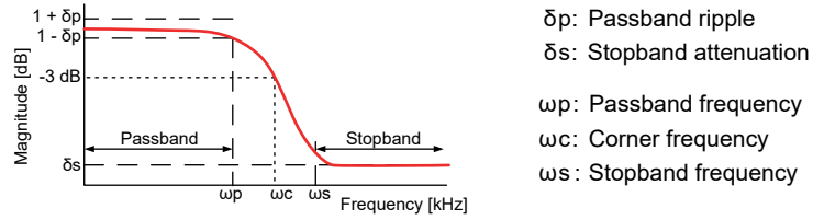
Figure 24: Butterworth Filter
