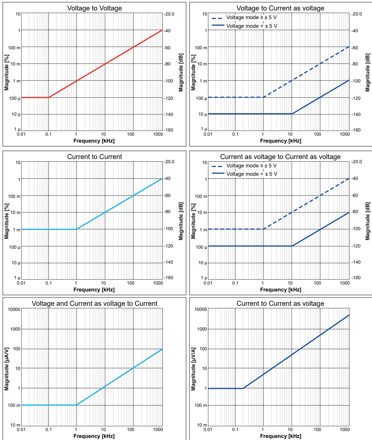
Figure 32: Representative Channel to Channel crosstalk
