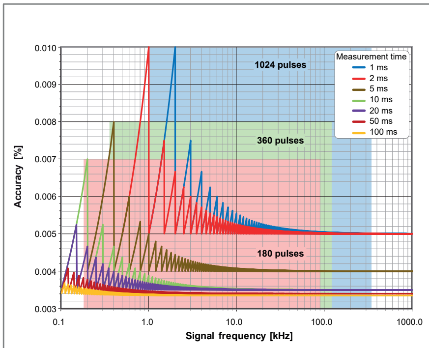
Figure 39: RPM sensor operating range versus inaccuracy and measurement time
