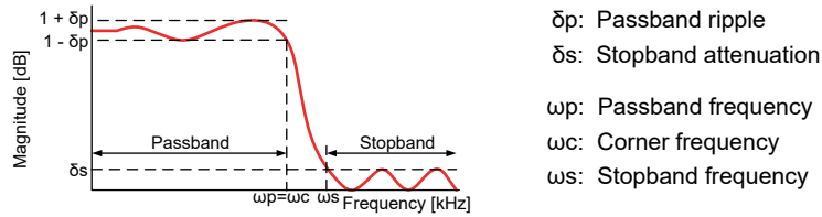
Figure 30: Digital Elliptic IIR Filter
