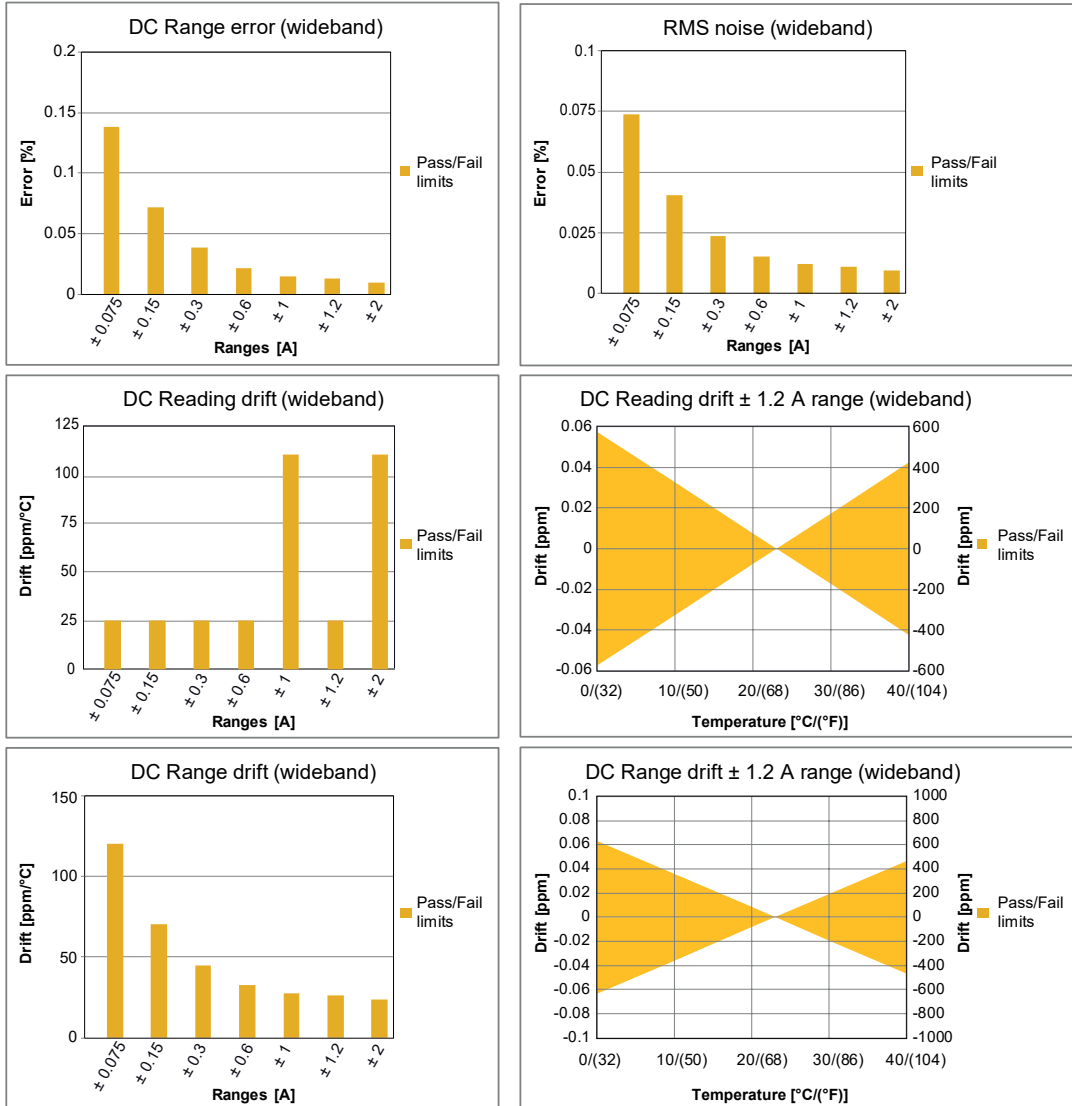
Figure 9: Wideband current mode specification
