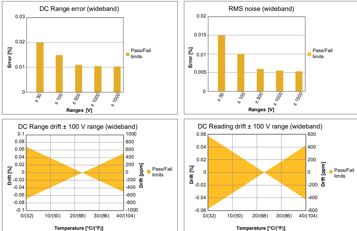
Figure 6: Wideband voltage specification
