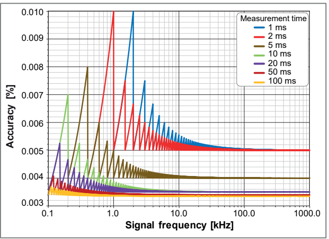
Figure 37: Maximum frequency inaccuracy
