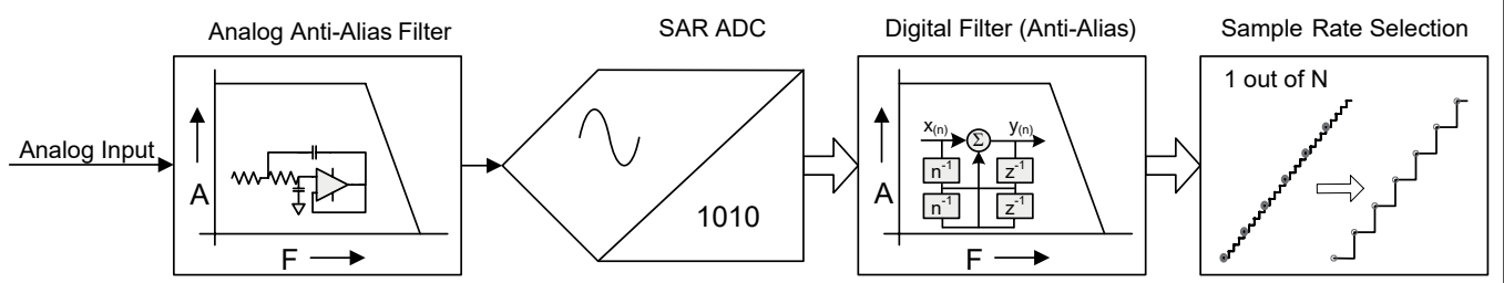
Figure 20: Combined analog and digital anti-alias filter block diagram
