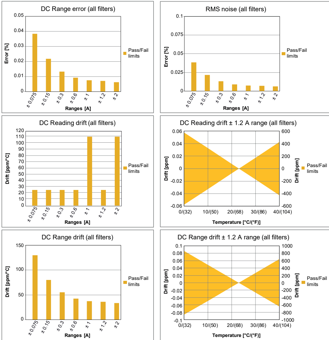
Figure 10: All filters used current mode specification
