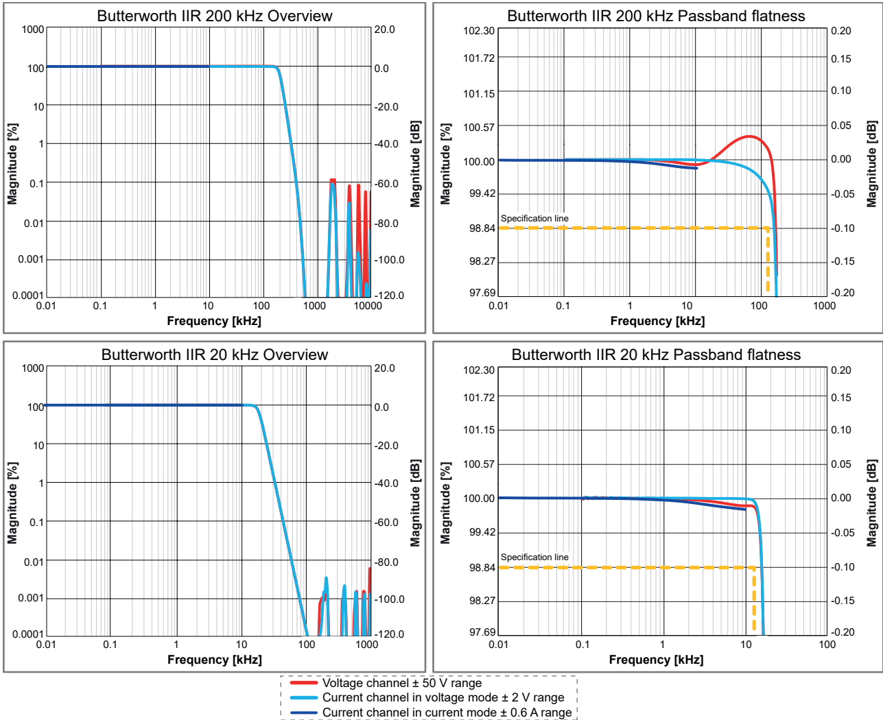
Figure 29: Representative Butterworth IIR examples (200 kHz for GN310B only; 20 kHz for GN310B and GN311B)
