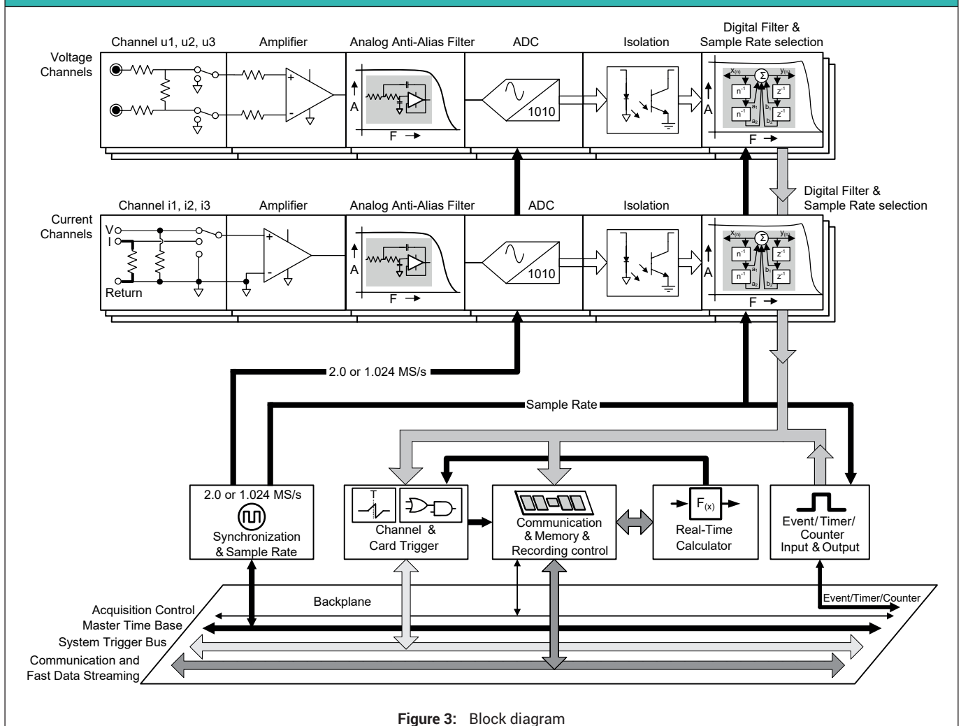
Figure 3: Block diagram
