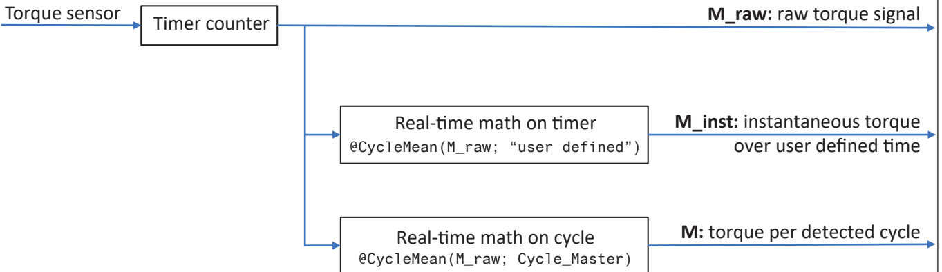
Figure 40: Simultaneous dynamic and accurate torque calculations
