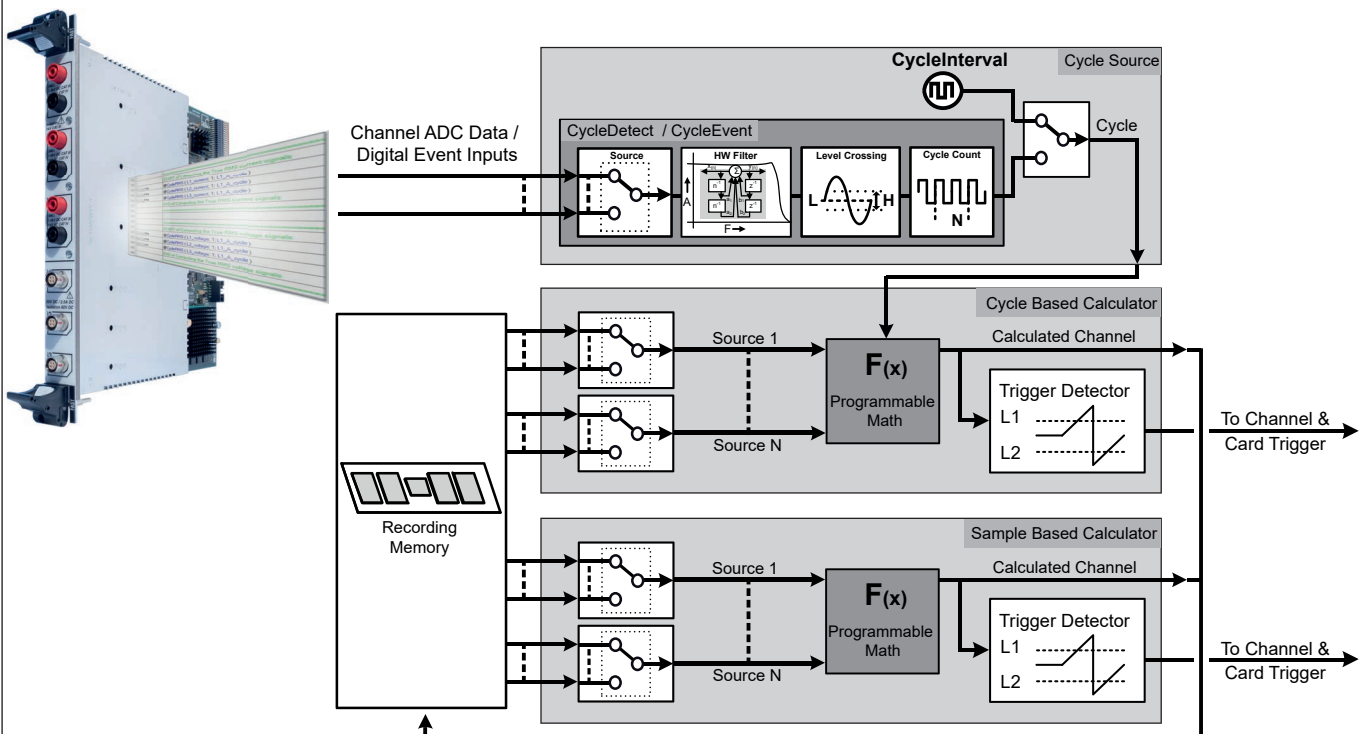
Figure 41: Real-time formula database (RT-FDB) calculators
