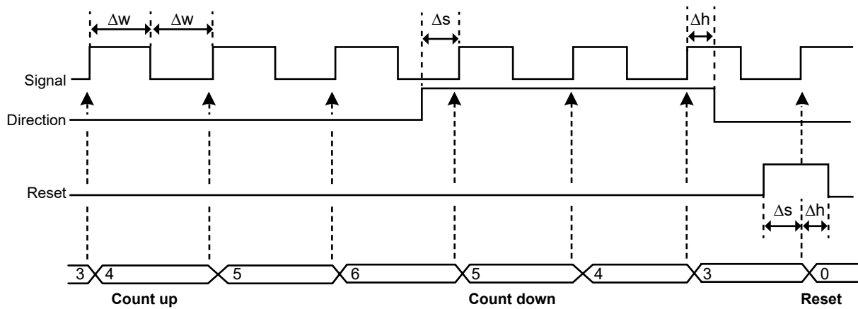
Figure 34: Uni- and Bi-directional timing
