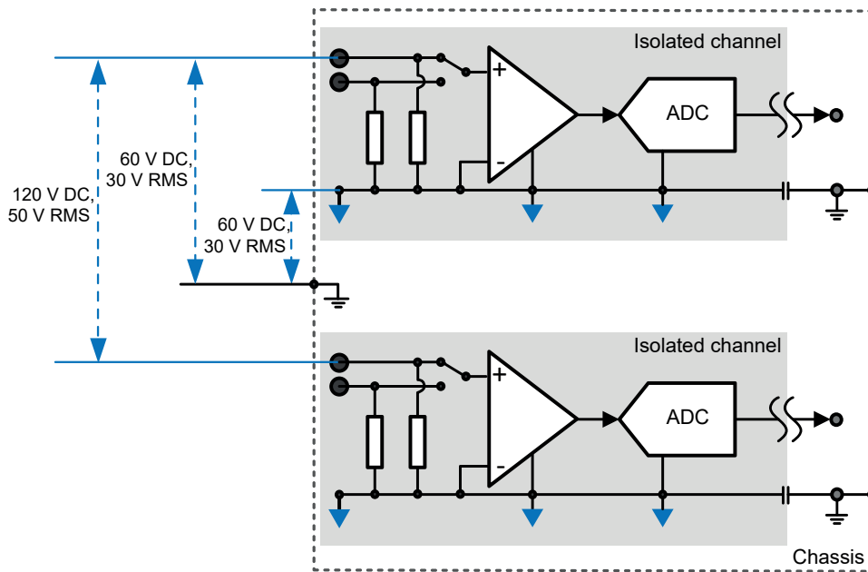
Figure 18: Current channels isolation ratings
