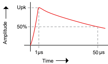
Figure 19: Example of 1.2/50 \mu s impulse
