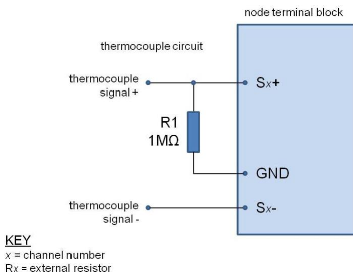
Figure 38 - Connecting a Thermocouple
