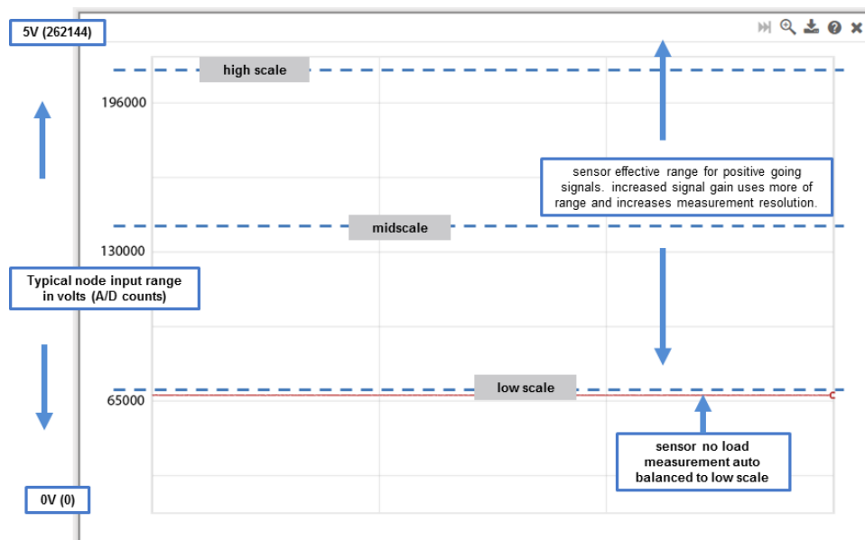
Figure 52 - Differential Input Resolution and Offset (18-bit Node)
