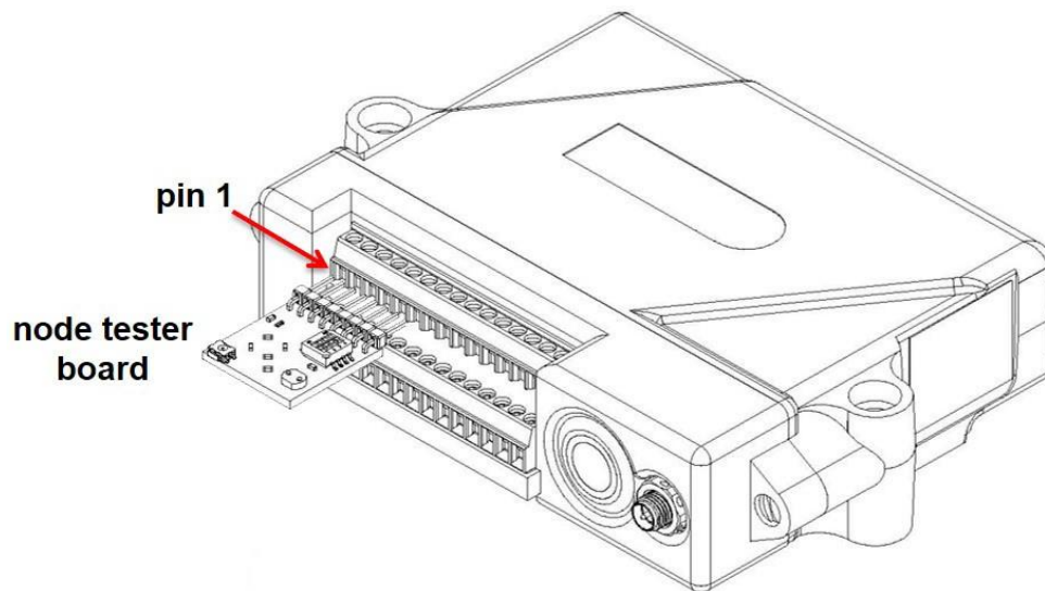
Figure 54 - Node Tester Board Installation
