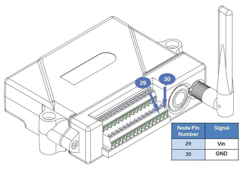
Figure 53 - External Power Connection
