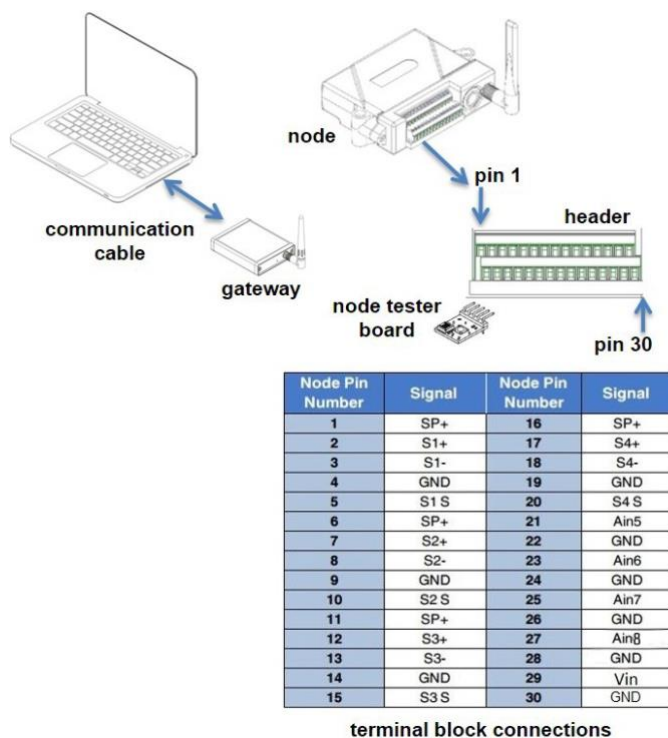
Figure 6 - System Connections
