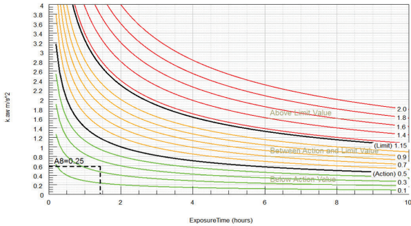
Whole Body Vibration: A(8) Daily Exposure Graph (Weighted RMS acceleration in m/s 2 ) Z Direction
