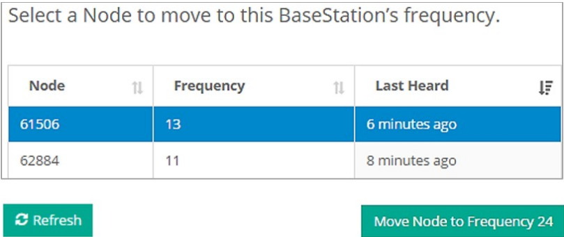
Figure 10 - Move Node
