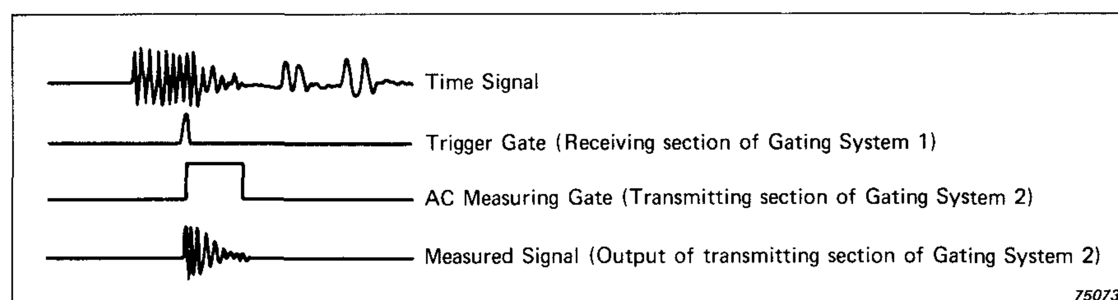
Fig.29. Setting of gates to measure early reflections with the instruments in Fig.28
