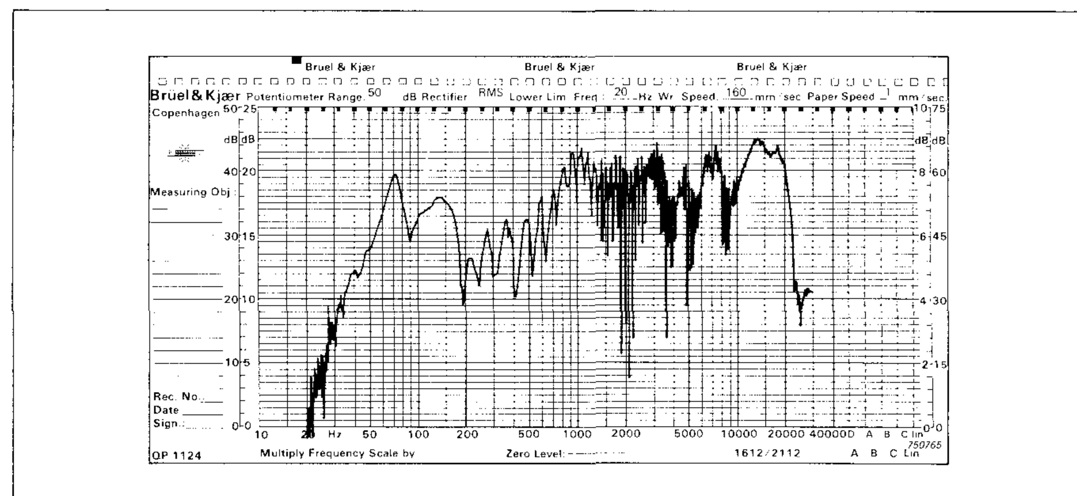
Fig.12. Frequency response of loudspeaker measured in a room with reflecting surfaces
