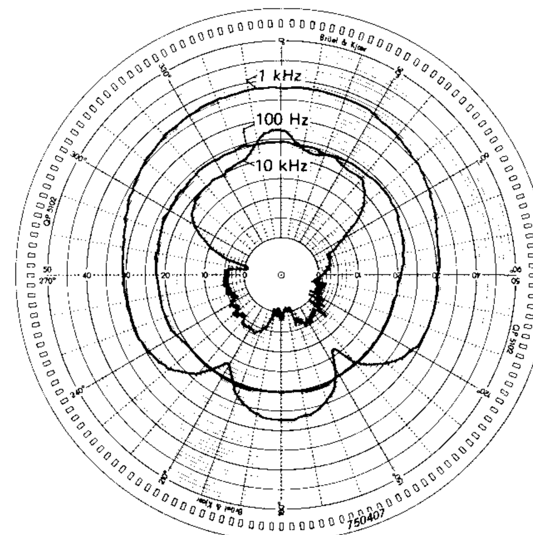
Fig. 15. Directional characteristics of the same loudspeaker measured with the Gating System in an anechoic chamber. The sharp dips and peaks are not as pronounced as for pure sine
