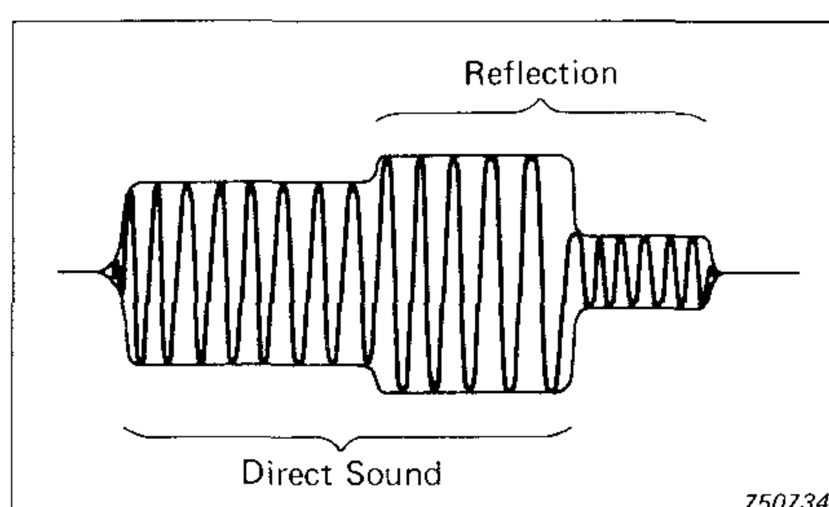
Fig. 7. Too long a burst results in overlap of the direct and reflected sound
