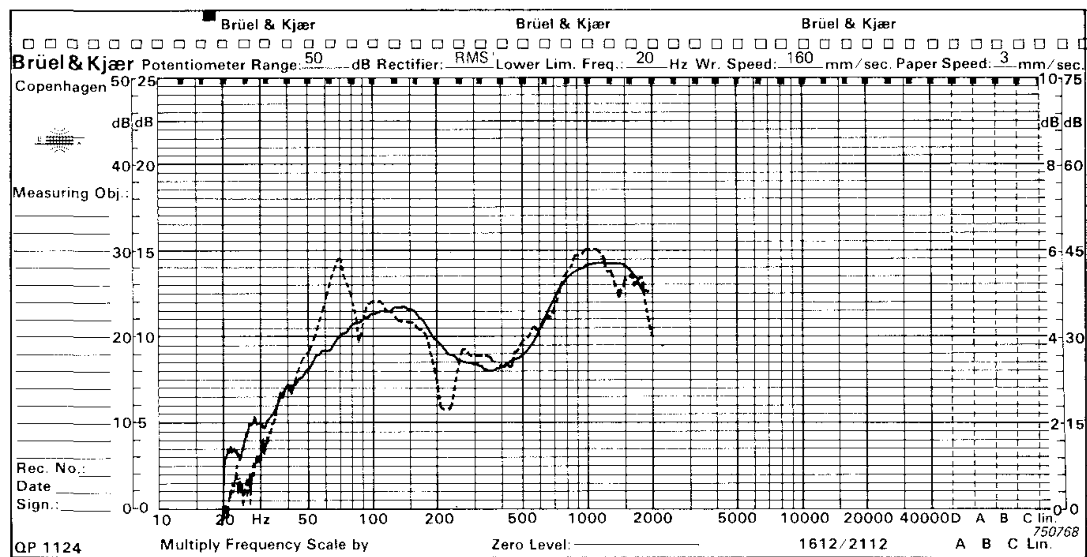
Fig.18. Illustration of averaging due to too short a tone burst. Dashed line shows free-field sine wave response, solid line shows the response measured with a tone burst consisting only of one period of its frequency
