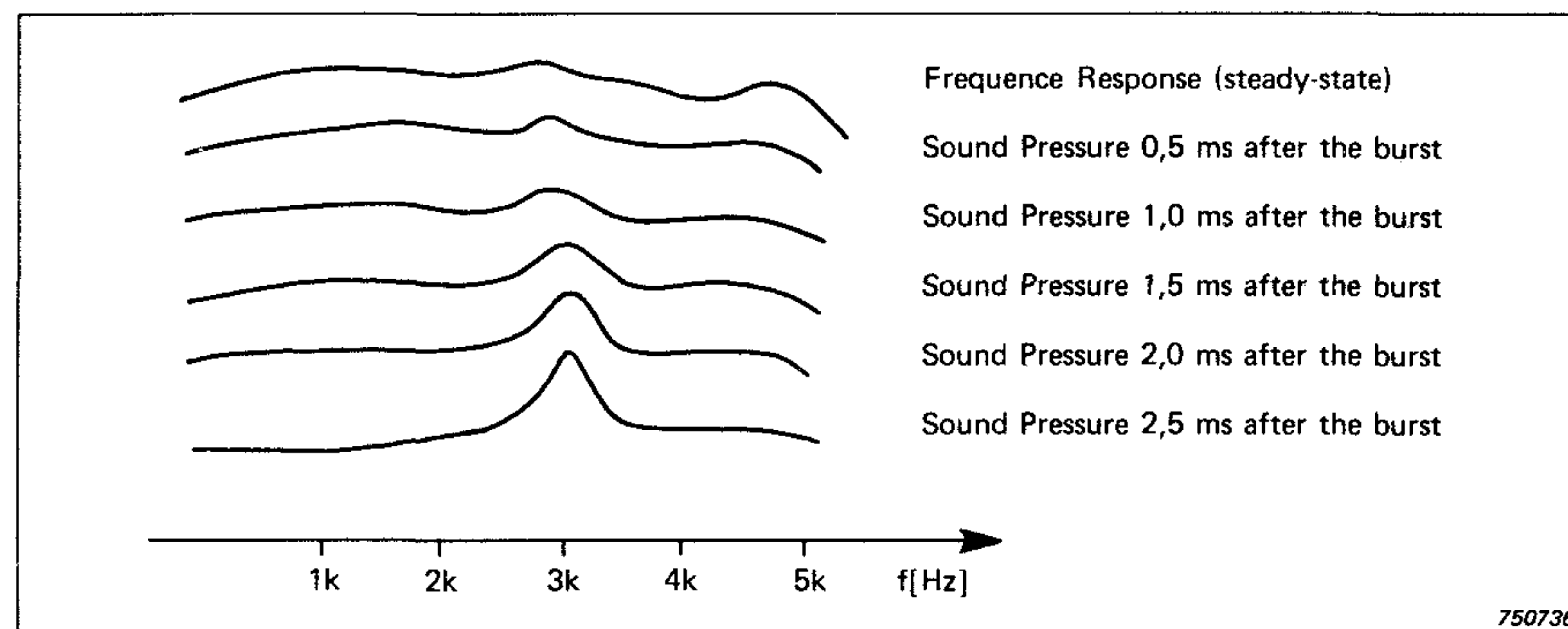
Fig.27. Frequency characteristics of early reflections compared to the steady state response
