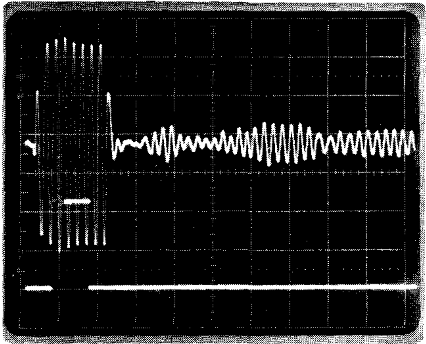
Fig.2. The gate is adjusted to include only the steady state portion of the signal
