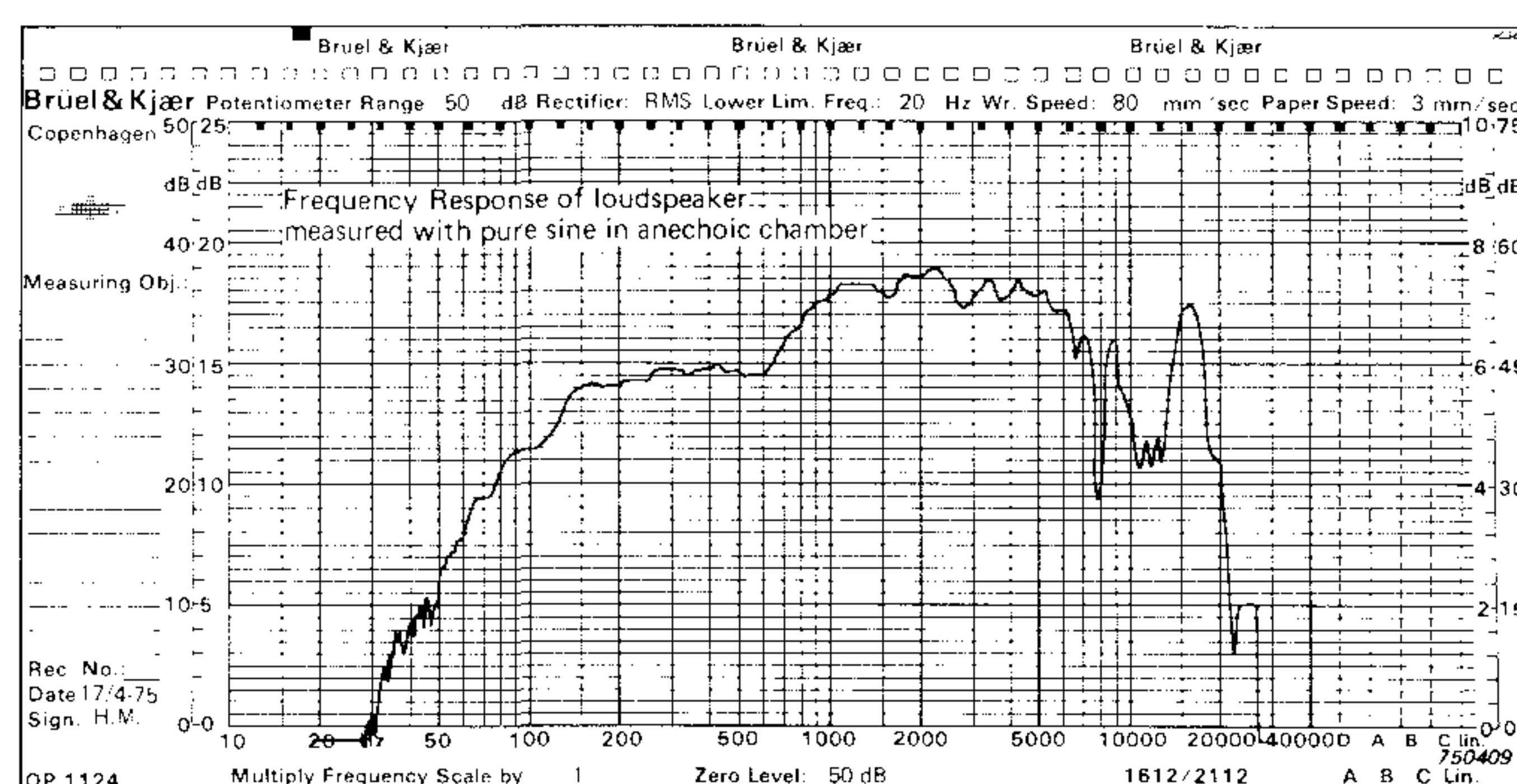
Fig.8. Frequency response of loudspeaker measured with pure sine in anechoic chamber
