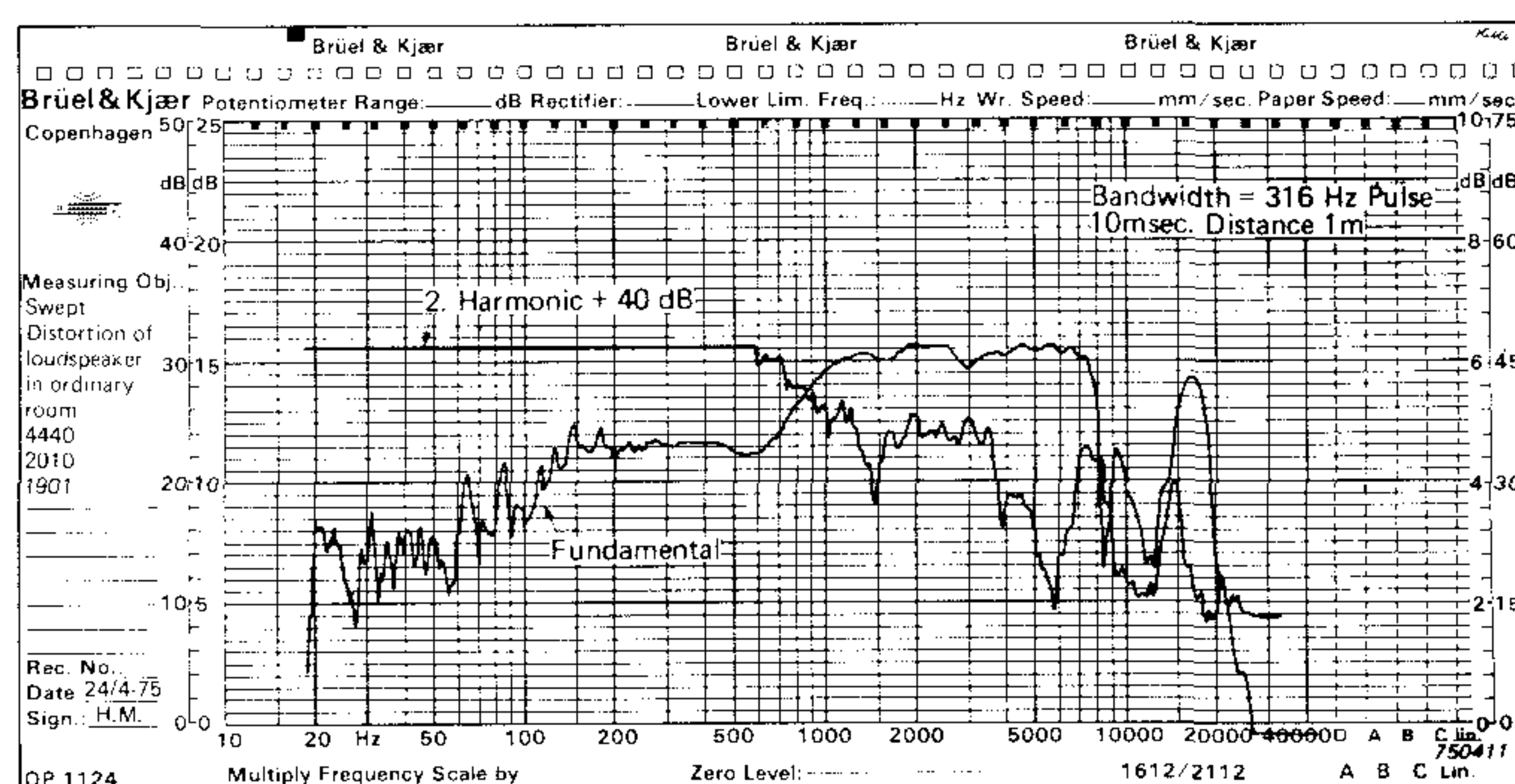
Fig.24. Results of distortion measurements. The top chart shows the fundamental and second harmonic of a loudspeaker measured with pure sines in a free-field. The lower chart shows the same measurements made with the Gating System in an ordinary room
