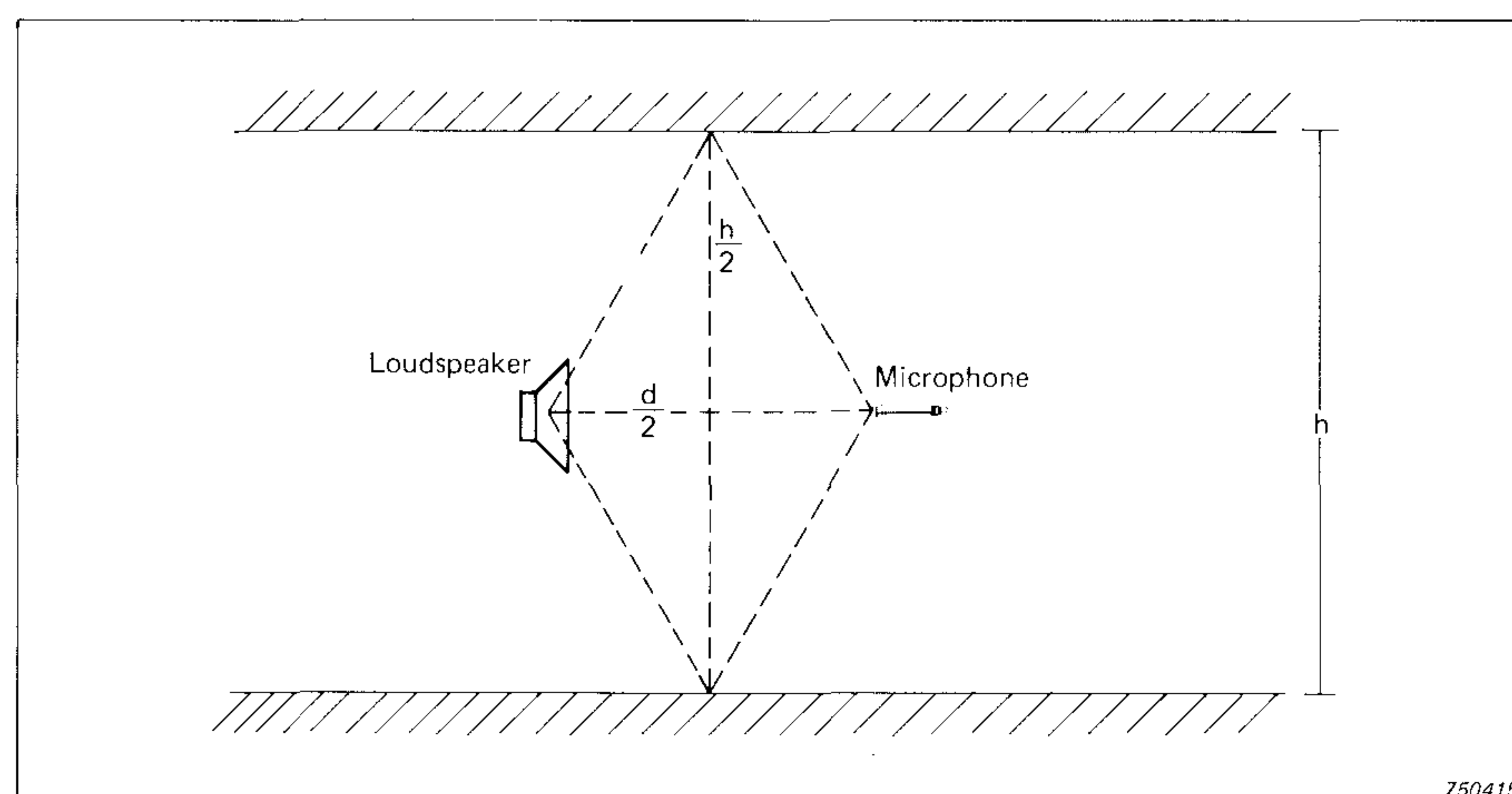
Fig.6. The microphone/loudspeaker combination should be centered in the room
