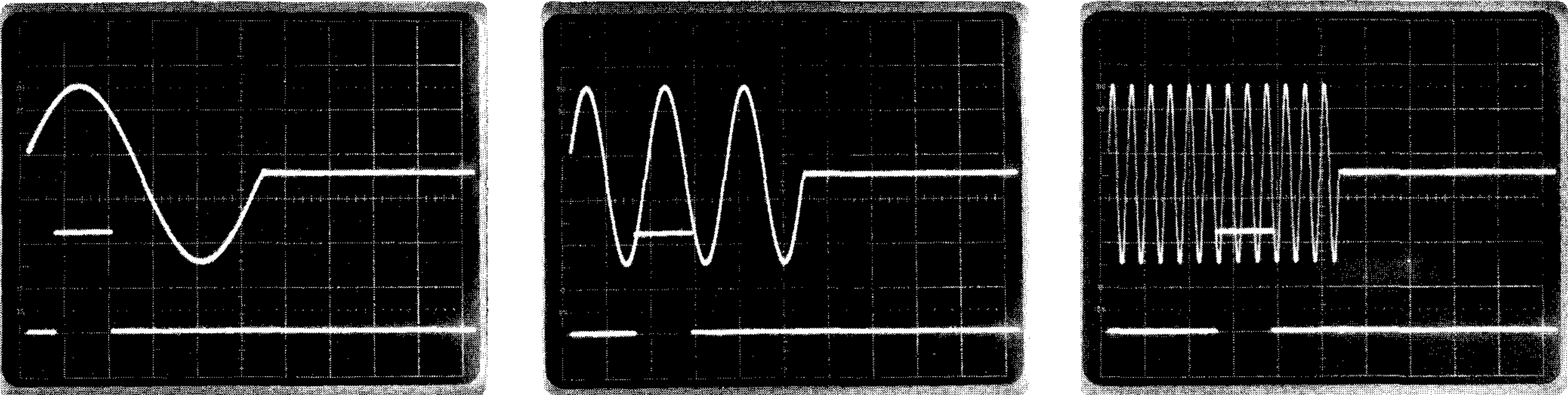
Fig.5. The tone burst always begins and ends with a positive-going zero crossing
