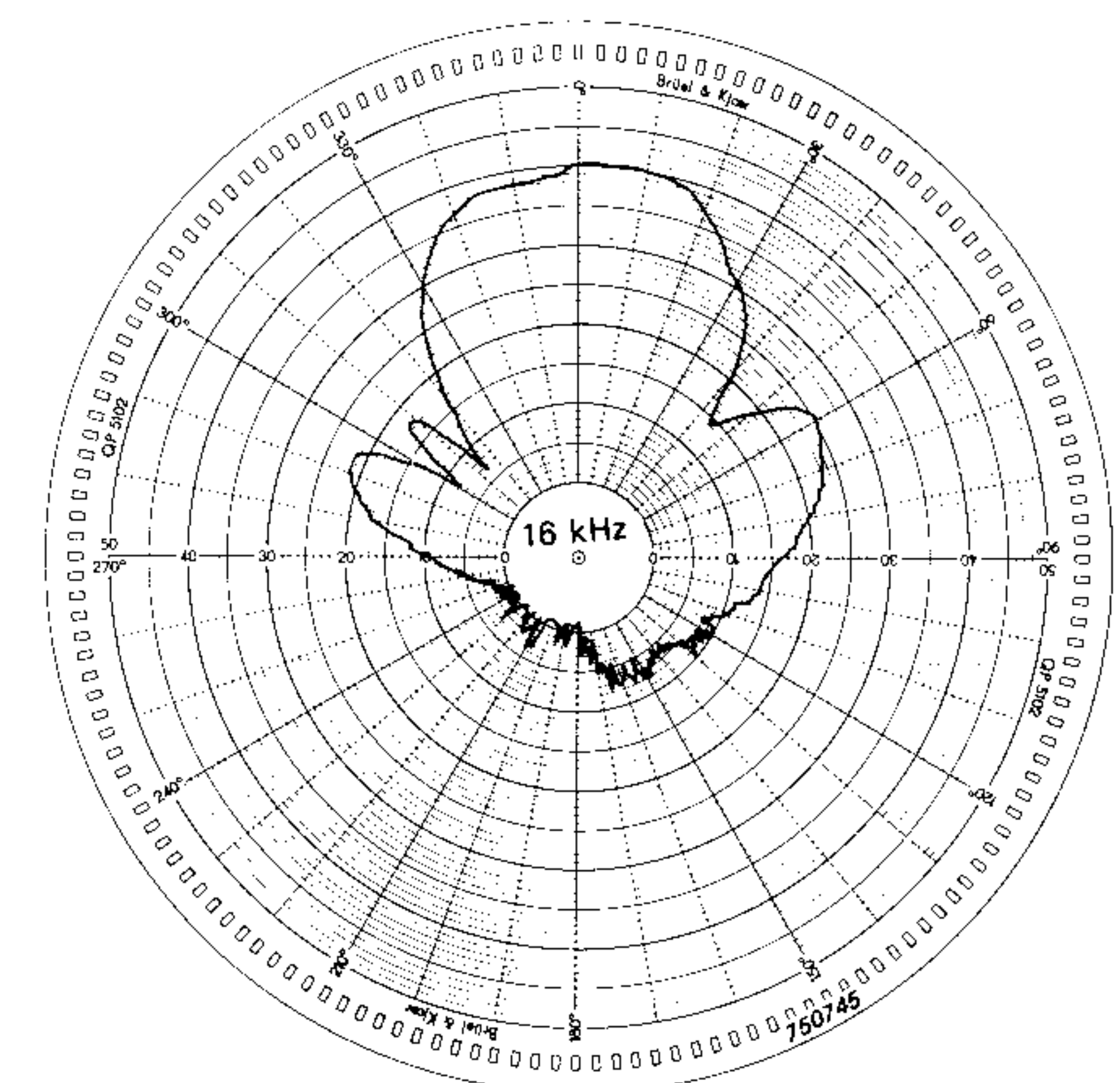
Fig.20. Reflections from door frame (Fig.19) are removed by use of the Gating System
