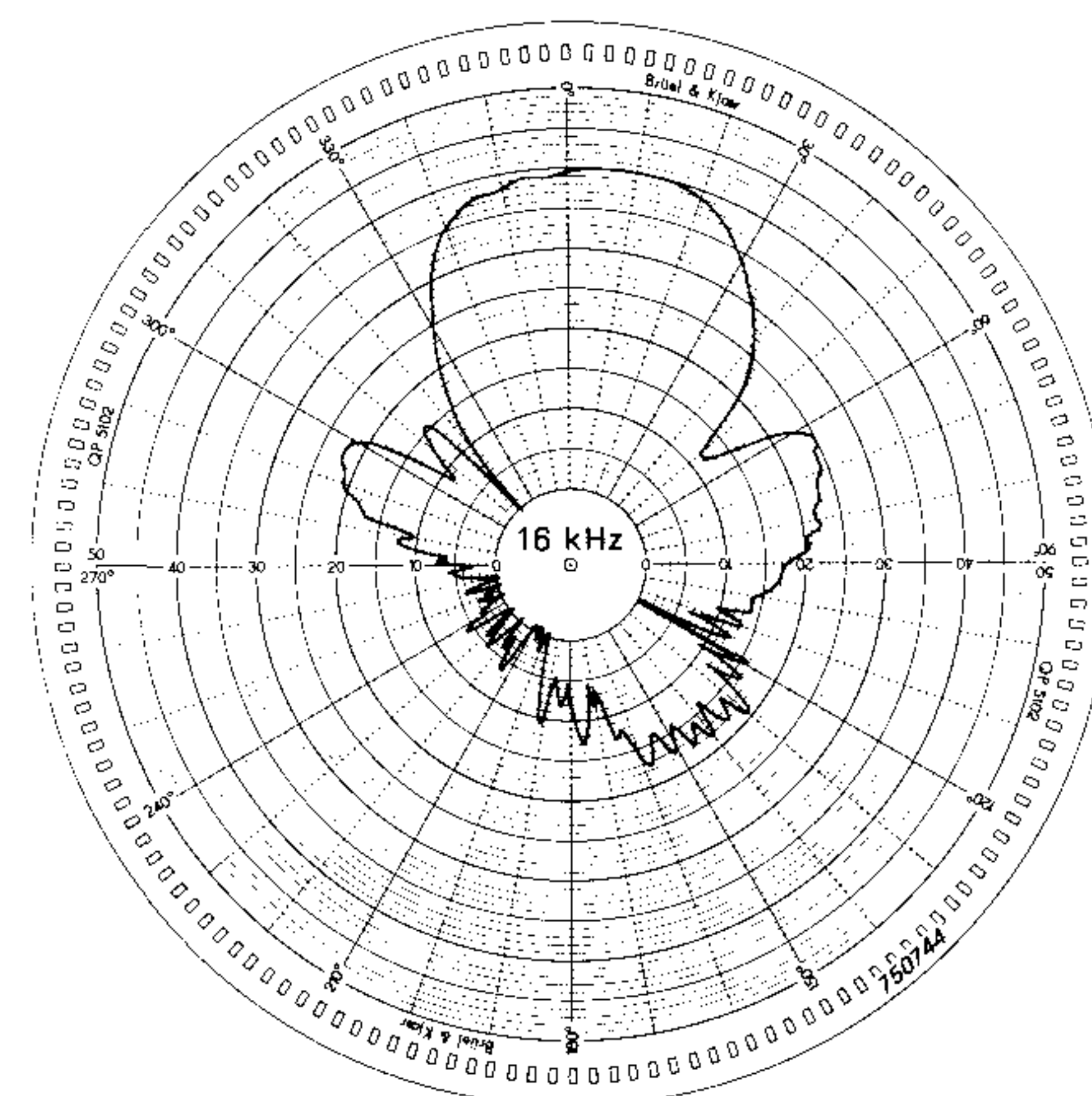
Fig.19. Directional characteristics of loudspeaker measured using pure sine in anechoic room. Note the influence of reflections from 120° to 170°. These reflections come from the door frame
