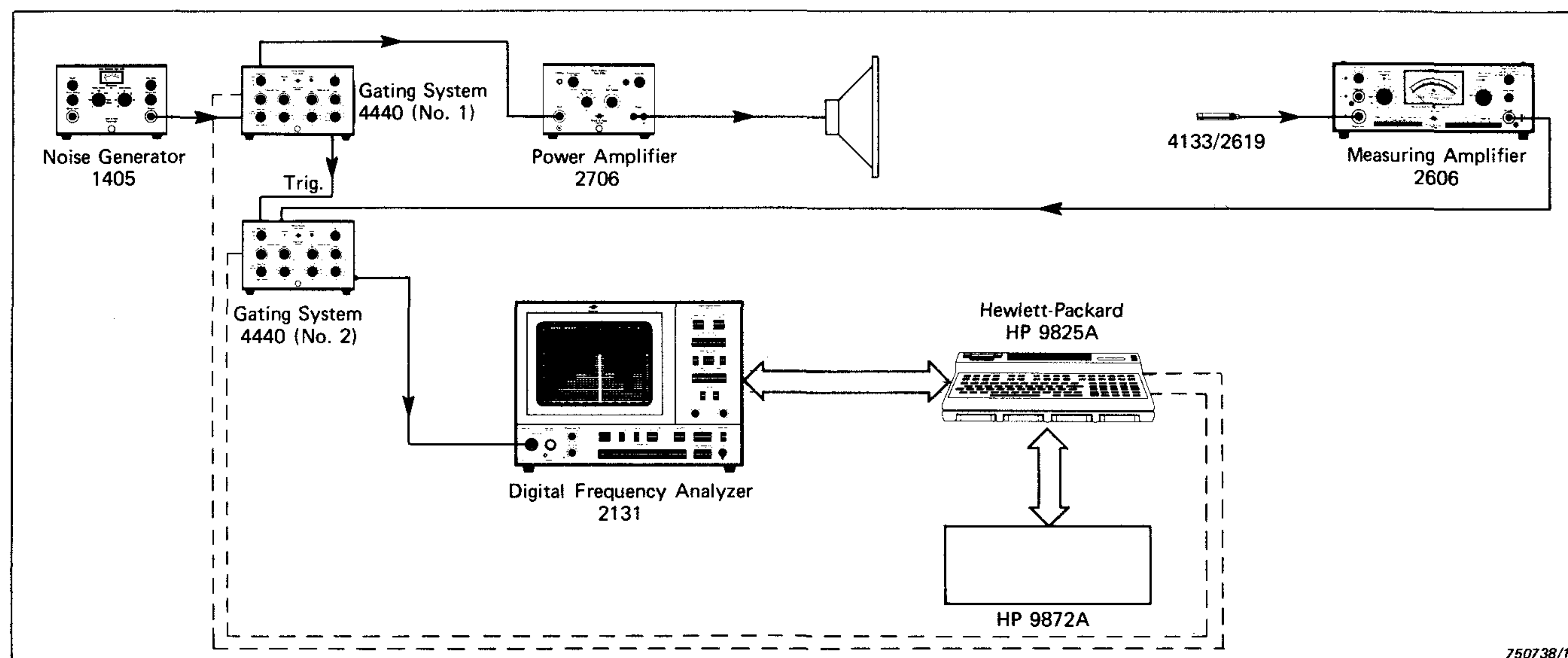
Fig.28. Instrument set-up for real-time analysis of early reflections using gated white noise
