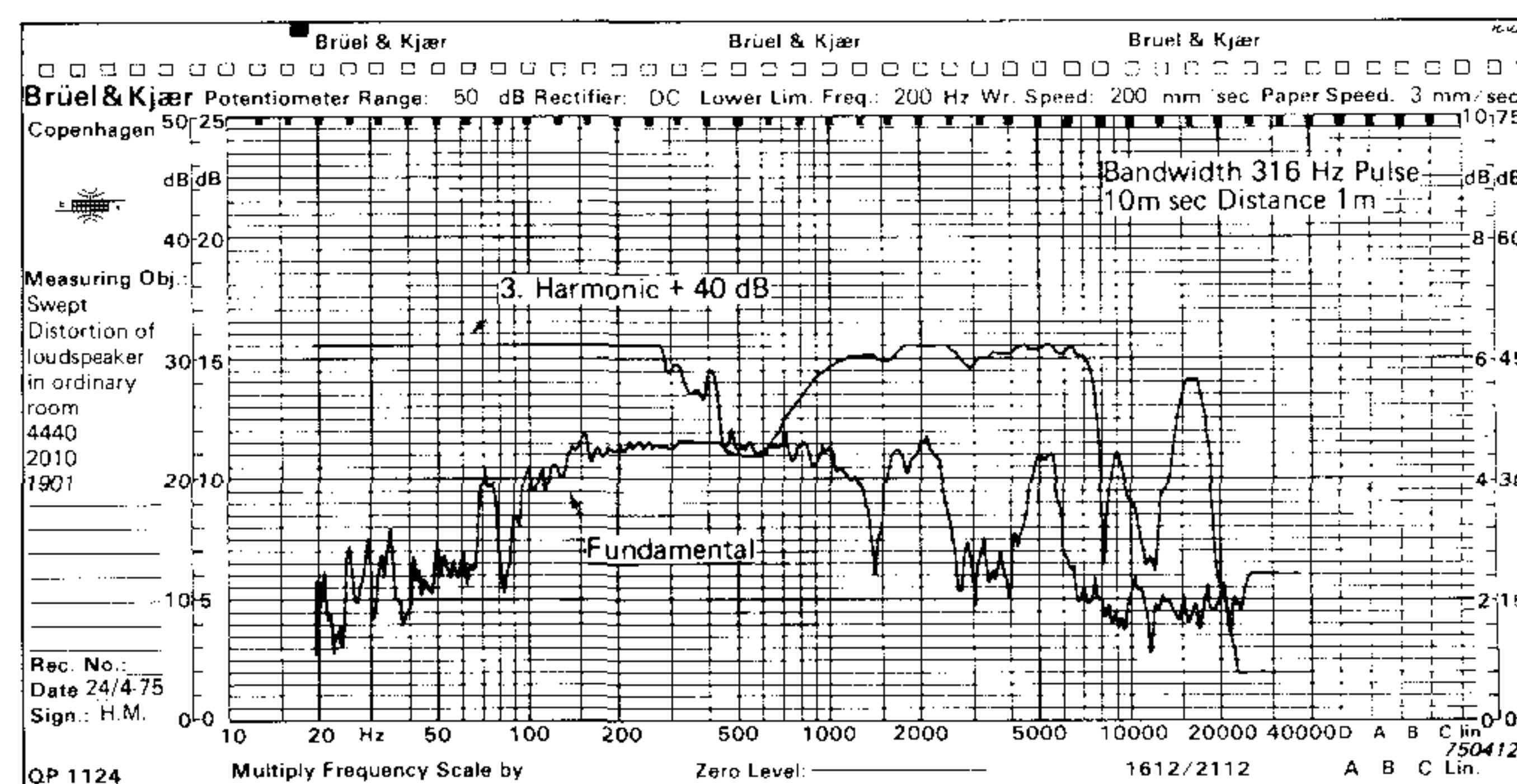
Fig.25. Results of distortion measurements. The top chart shows the fundamental and third harmonic of a loudspeaker measured with pure sines in a free-field. The lower chart shows the same measurements made with the gating System in an ordinary room
