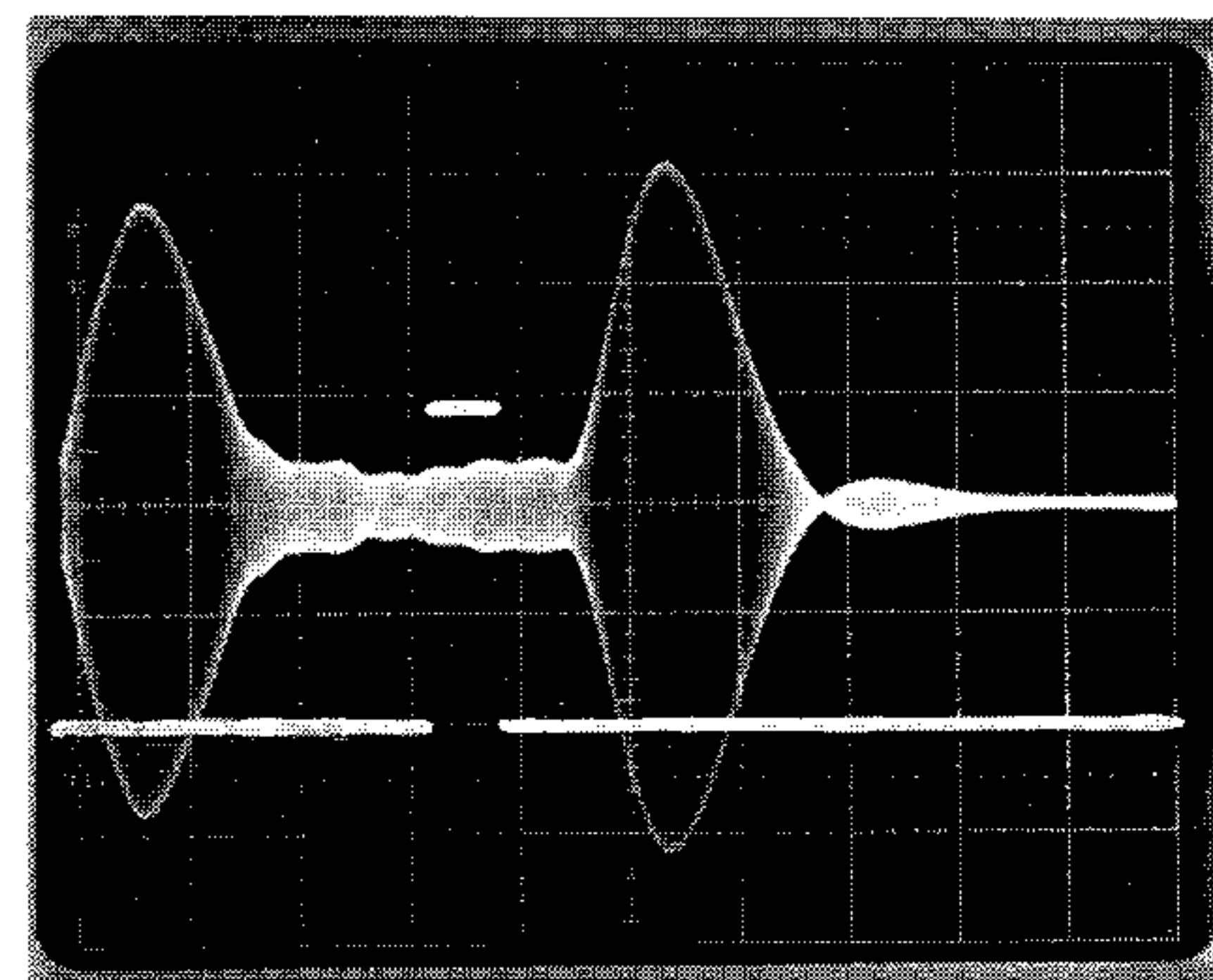
Fig.22. Response of filter tuned to second harmonic of the tone burst. Gate is adjusted to measure distortion component
