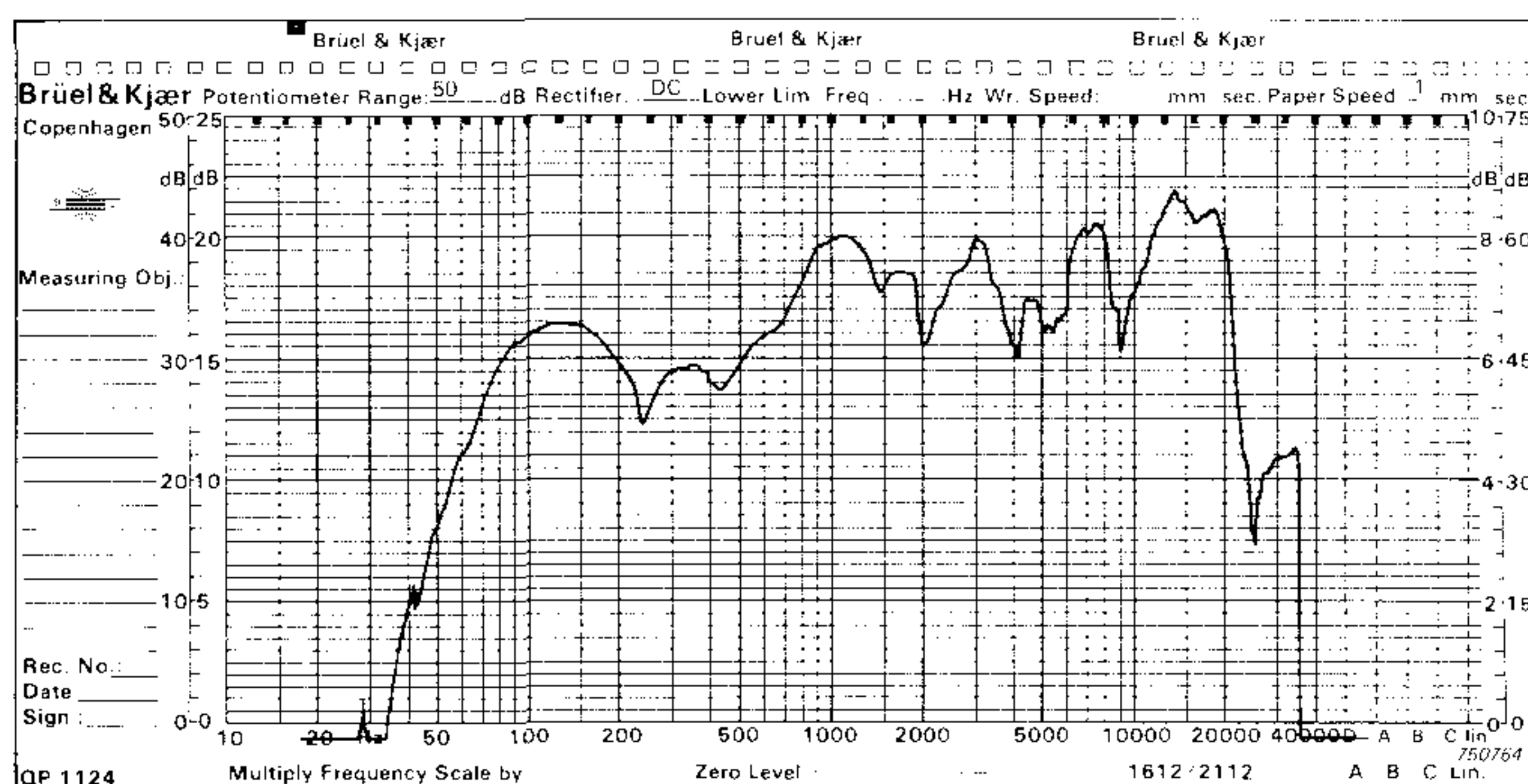
Fig.10. Frequency response of the loudspeaker in Fig.11 measured with Gating System in anechoic room. The difference between these two curves indicates the influence of the Gating System
