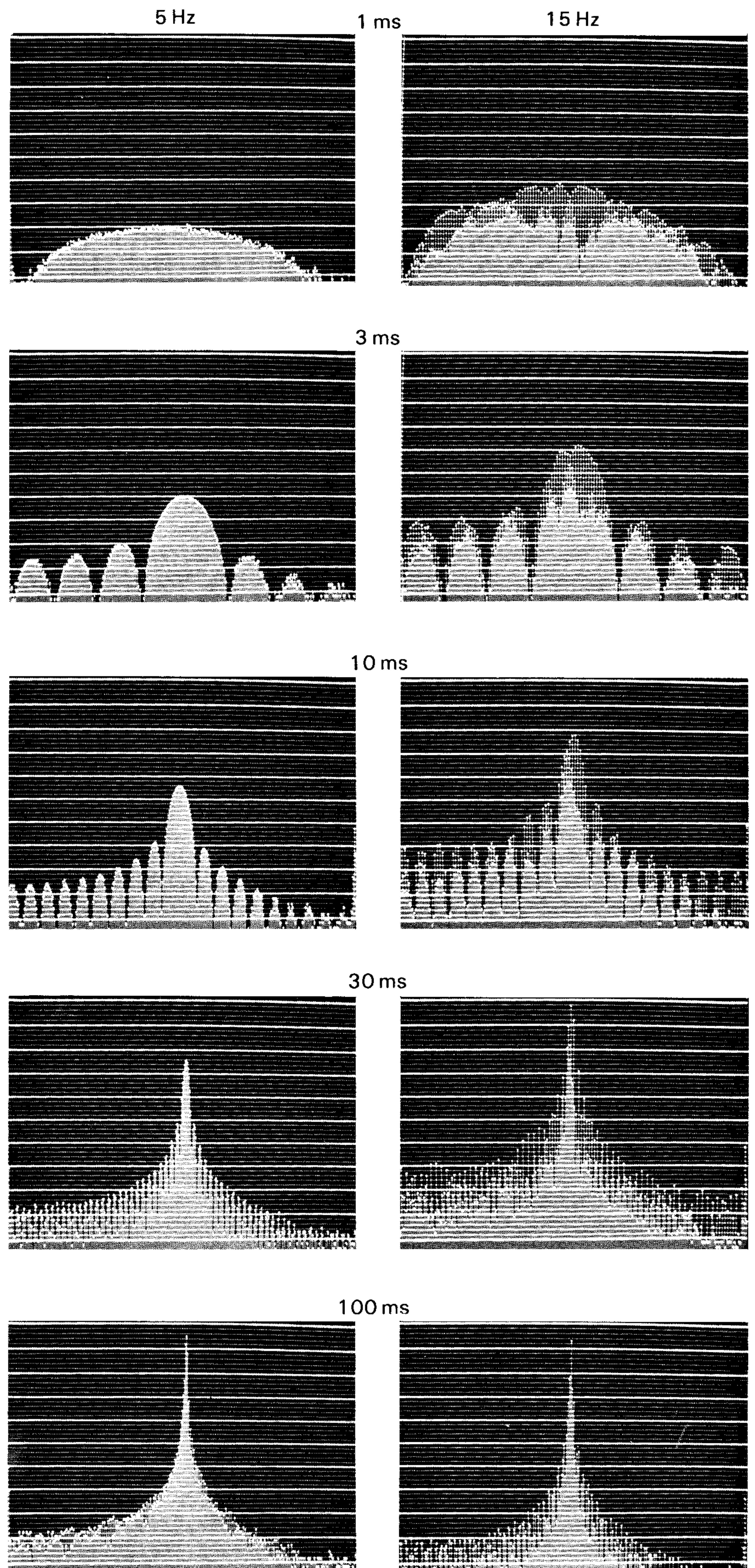
Fig.17. Frequency spectra of tone burts with Repetition Rates of 5 Hz and 15 Hz. Burst width varies from 1 ms to 100 ms. Center frequency is 1 kHz. Displayed on linear scale from 0 to 2 kHz with a 50 dB vertical scale
