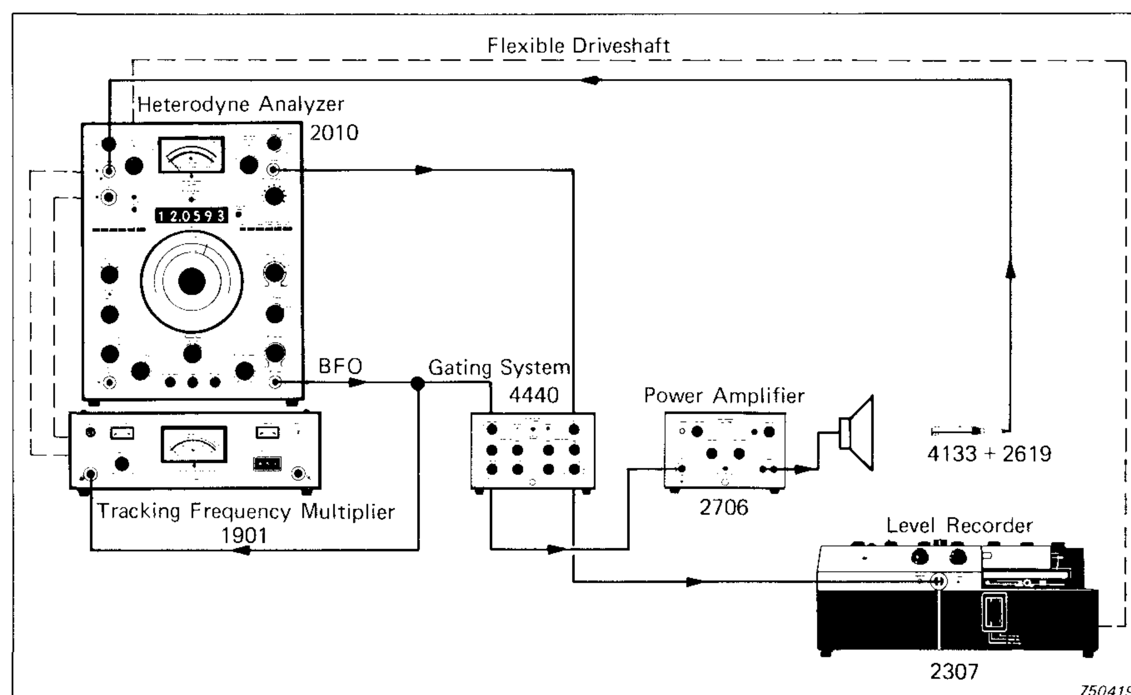
Fig.23. Instrument set-up for distortion measurements using the Gating System
