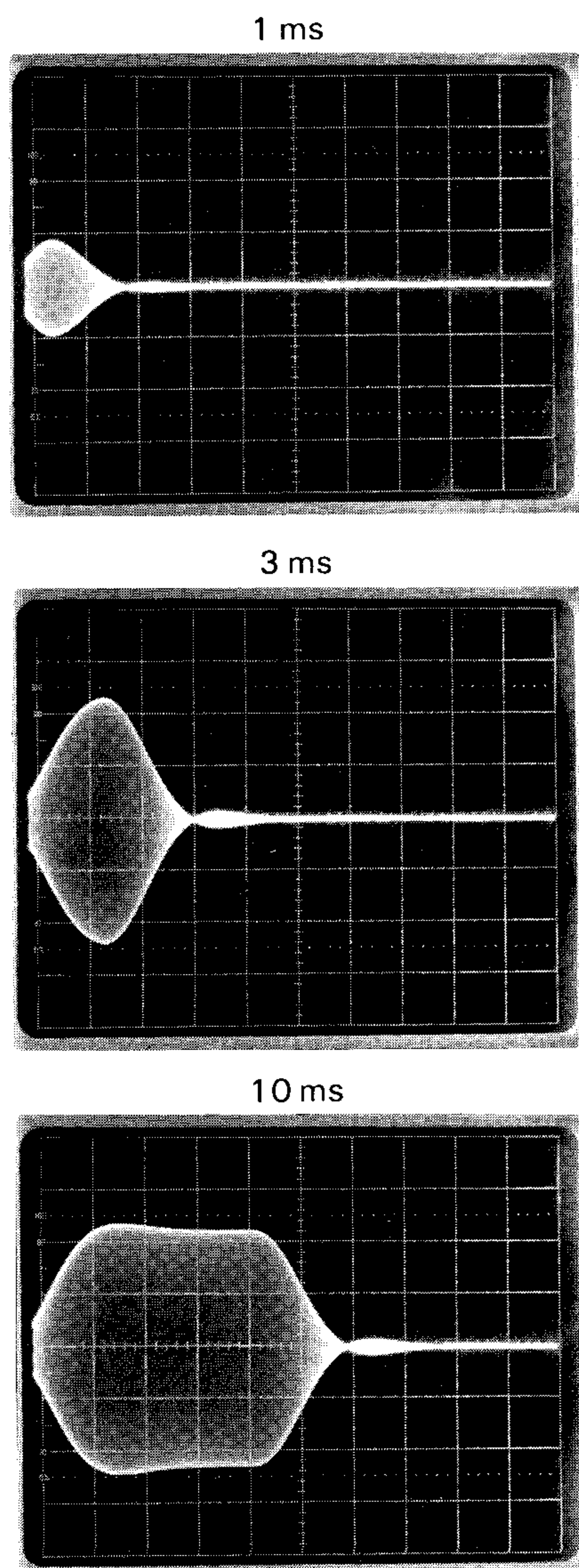
Fig.21. Response of 316 Hz wide filter to various tone burst durations
