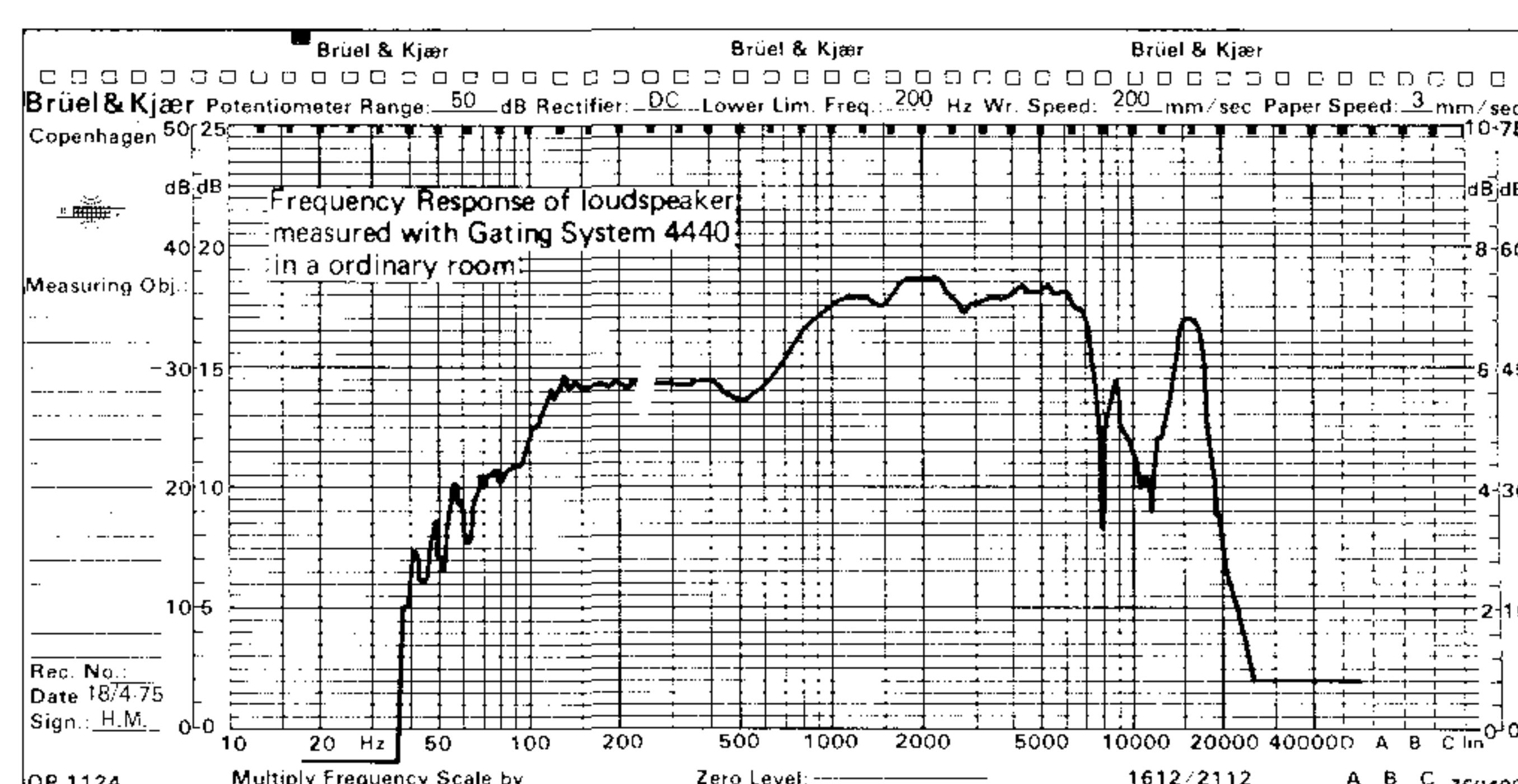
Fig.9. Frequency response of the same loudspeaker measured with the Gating System
