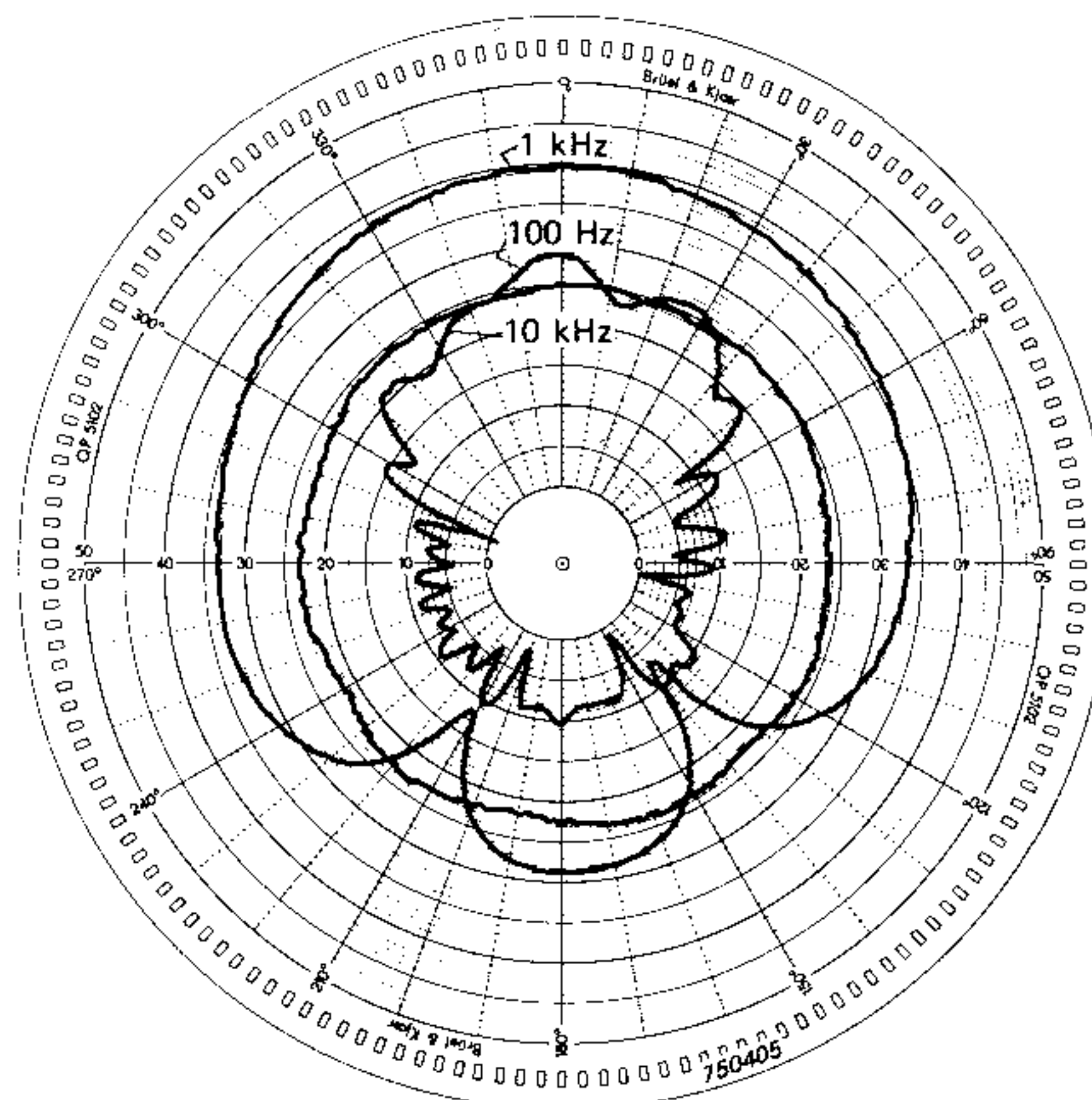
Fig. 13. Directional characteristics of loudspeaker measured with pure sine in anechoic chamber
