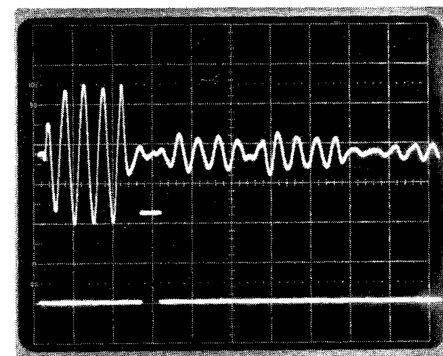
Fig.26. Adjustment of the gate for measurement of early reflections
