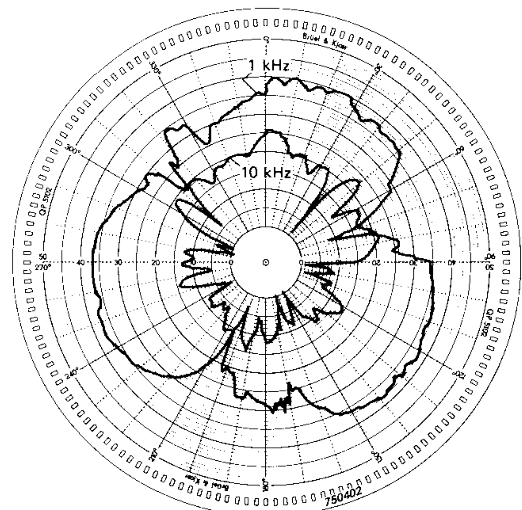
Fig. 16. Directional characteristics of the same loudspeaker measured with pure tones in ordinary room
