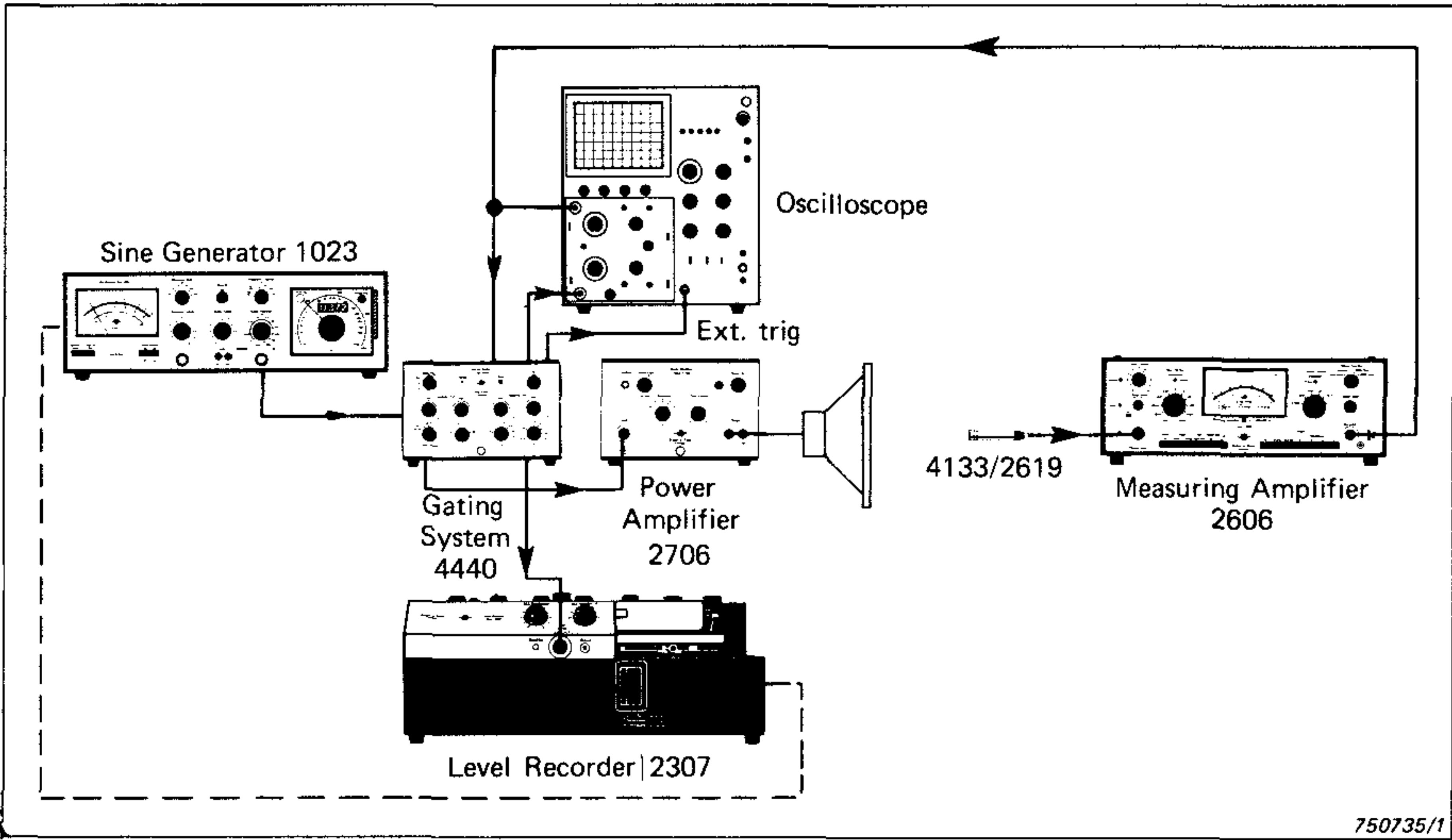
Fig.3. Instrument set-up using the Gating System
