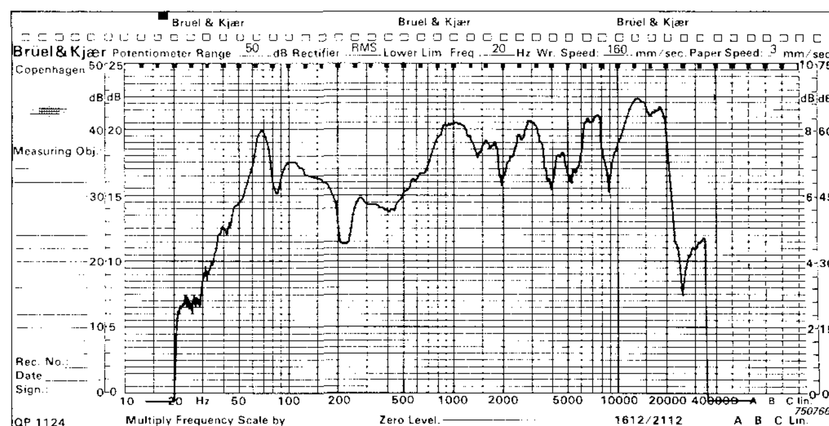
Fig.11. Frequency response of a loudspeaker (not the same as in Figs.8 and 9) using pure sine in anechoic room
