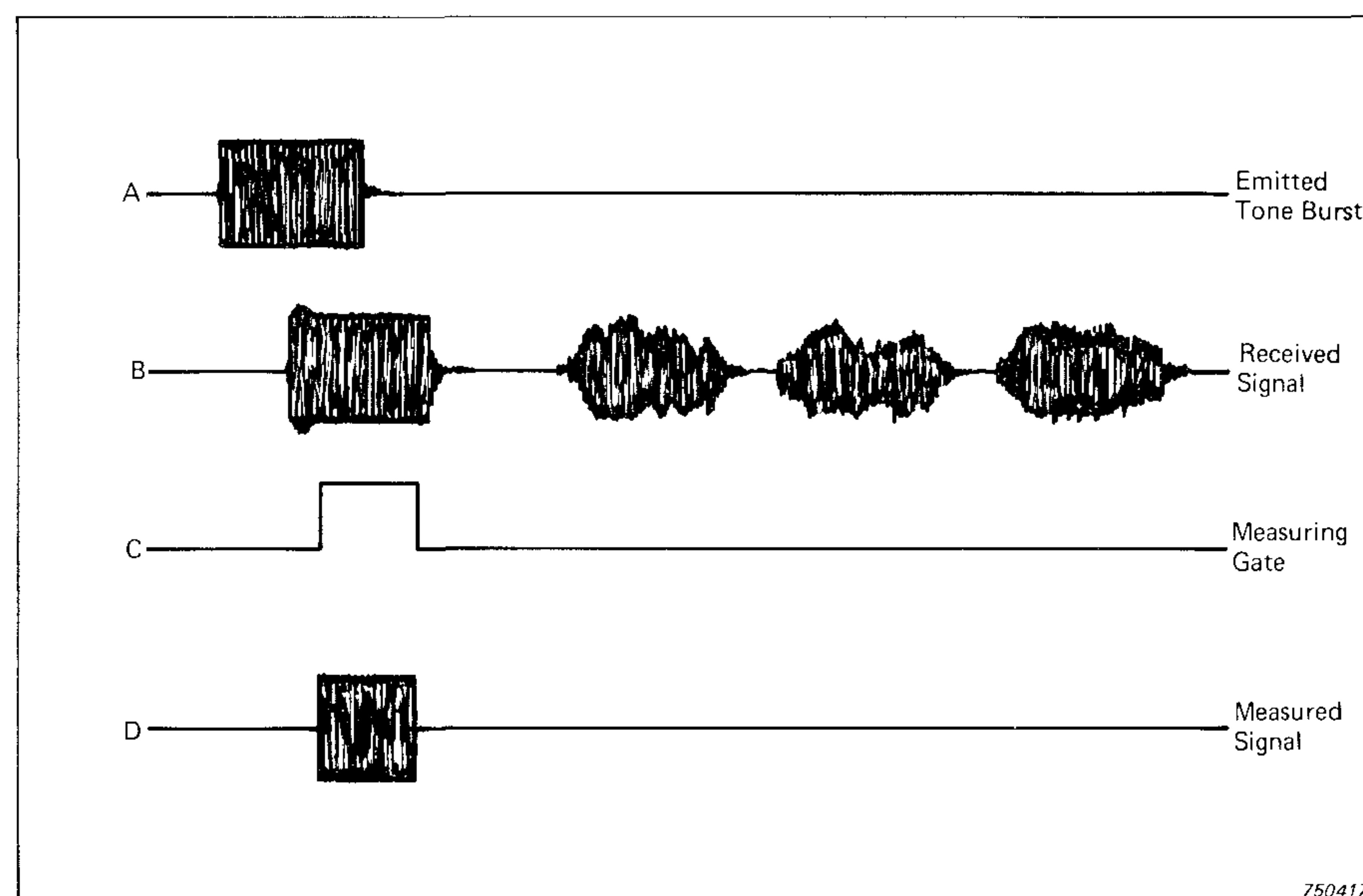
Fig.1. Principle of the Gating System
