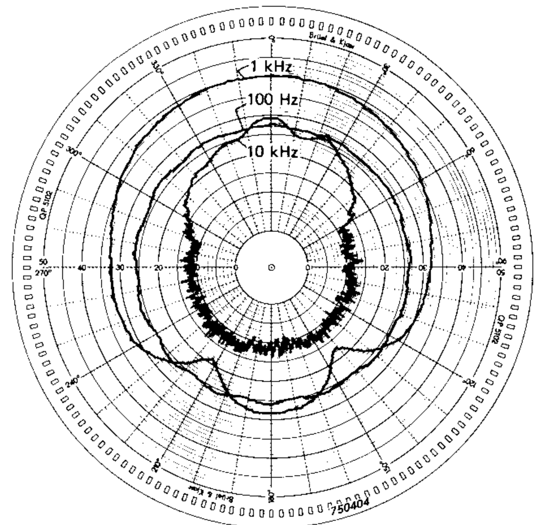
Fig. 14. Directional characteristics of the same loudspeaker measured with the Gating System in an ordinary room. Note the 10 kHz curve shows the background noise level of the room
