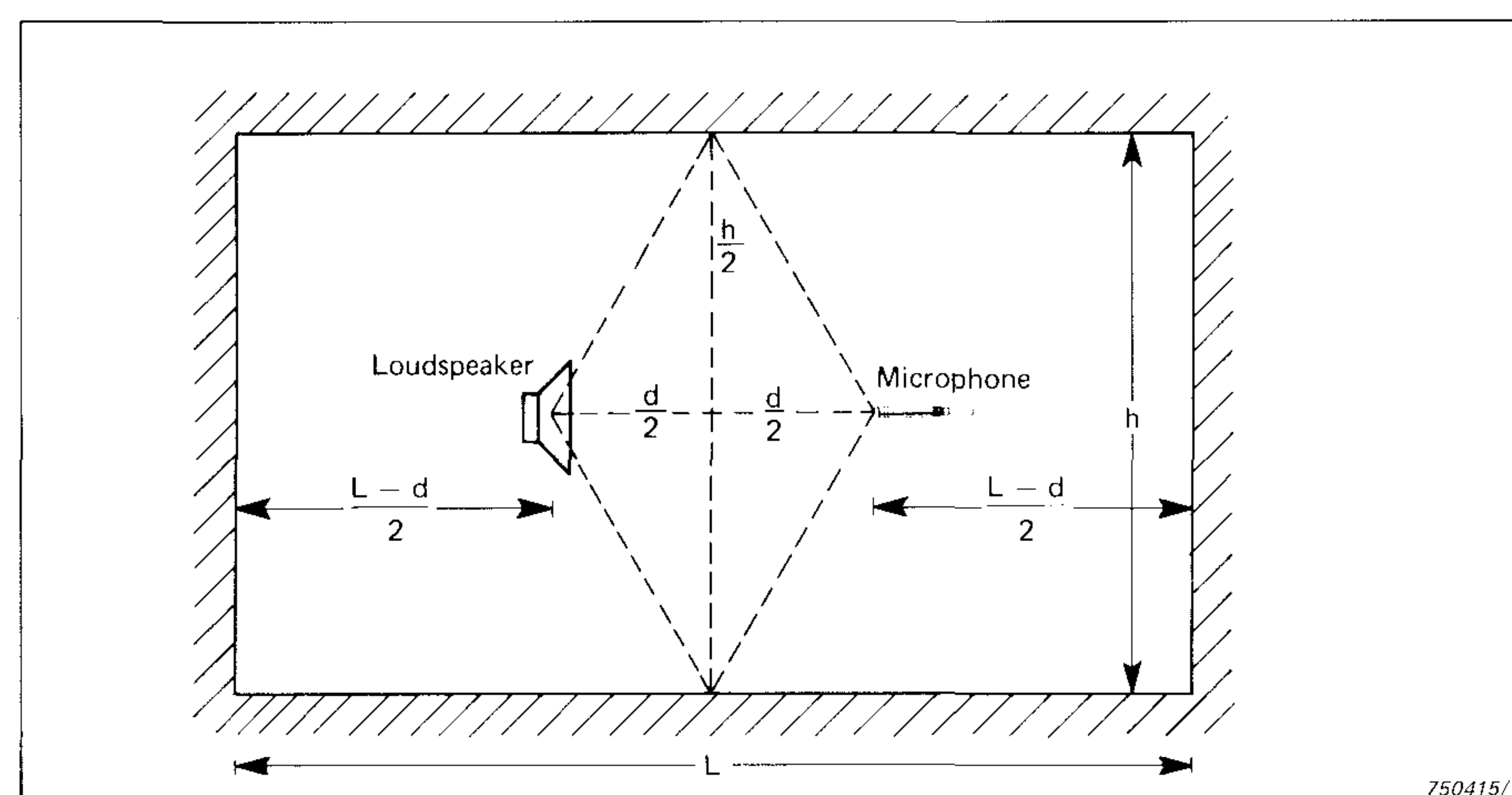
Fig.30. Travel distances for the first reflections when the loudspeaker and microphone are centered along all three axes of the room
