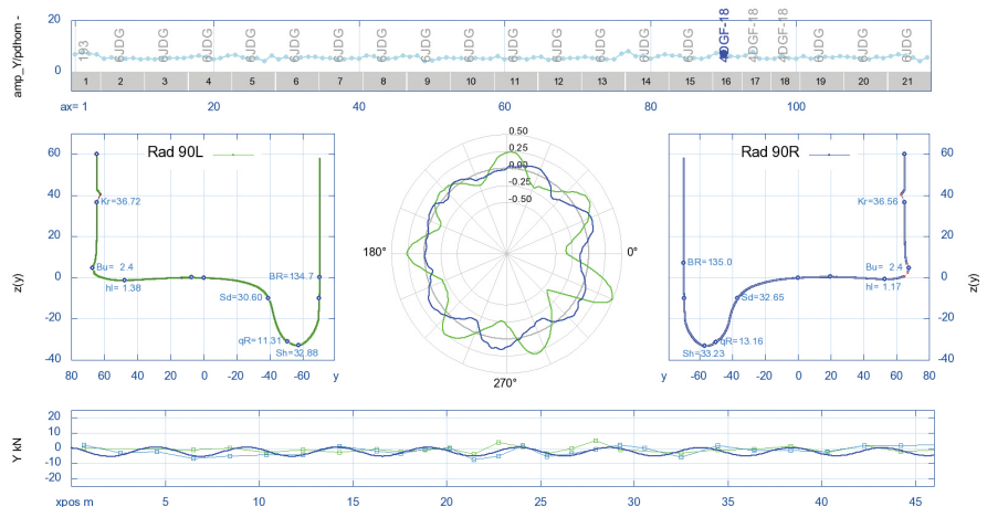
Running behaviour
